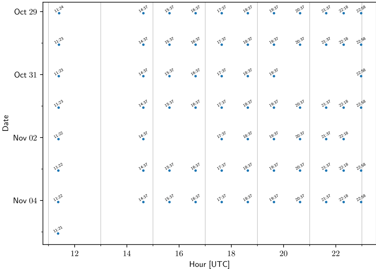
TEMPO sample times: LoganUT
