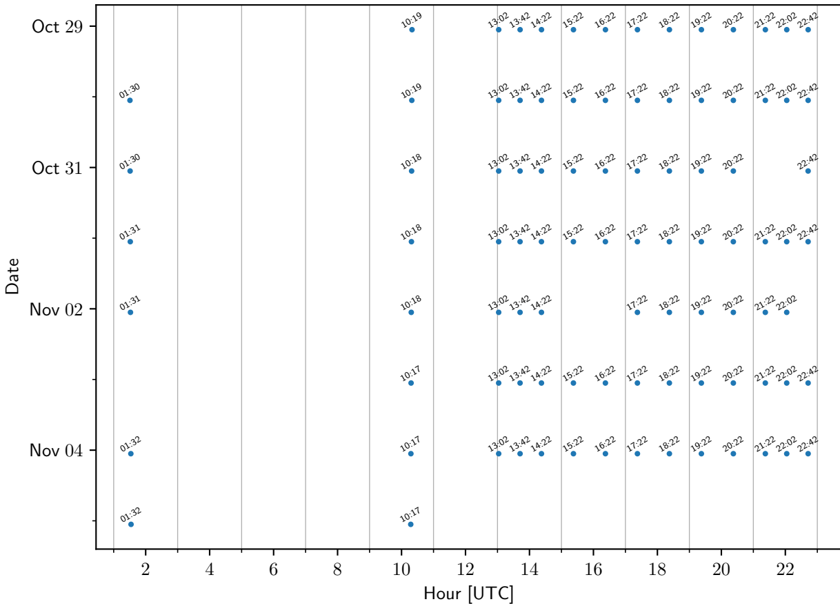
TEMPO sample times: CameronLA
