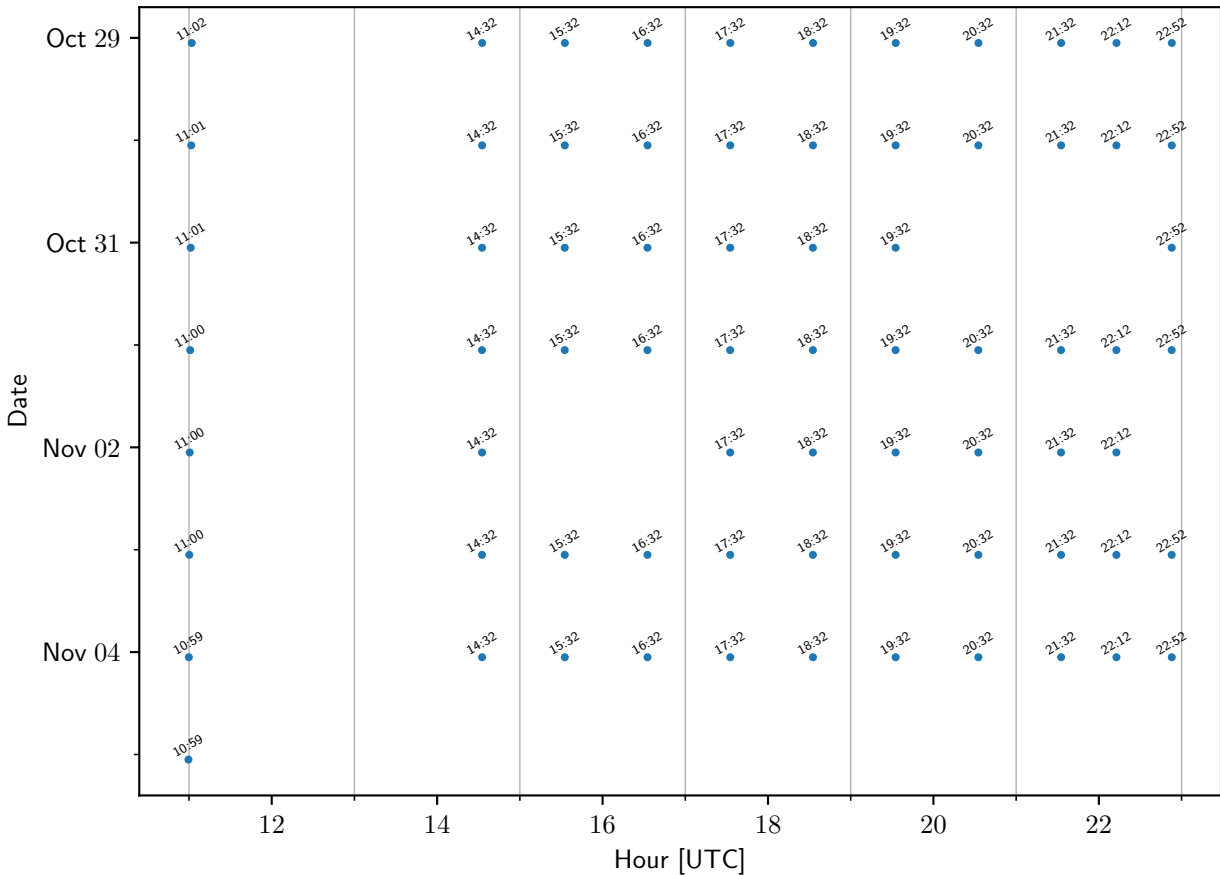
TEMPO sample times: ECCC
