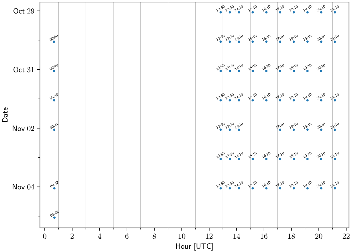
TEMPO sample times: PittsburghPA
