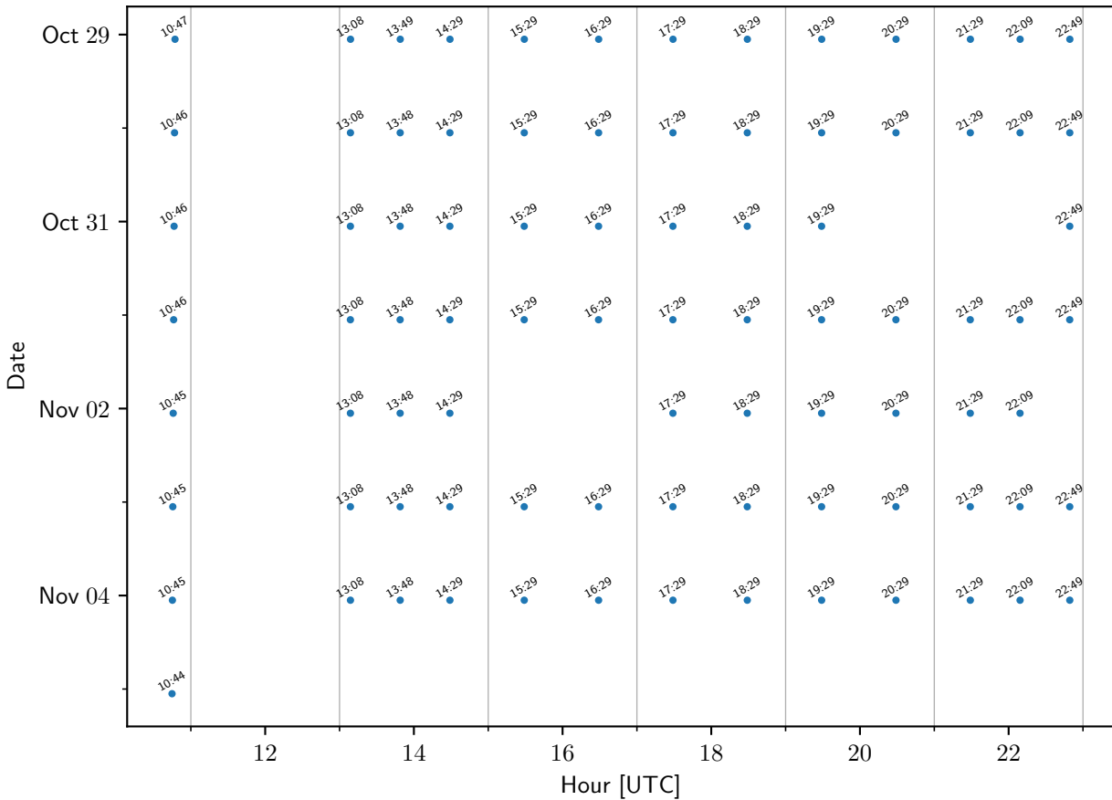
TEMPO sample times: Altzomoni
