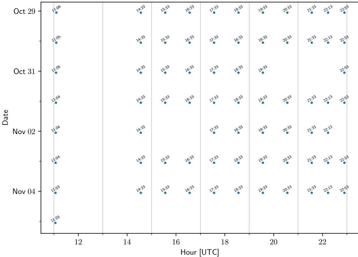
TEMPO sample times: Roswell11NM
