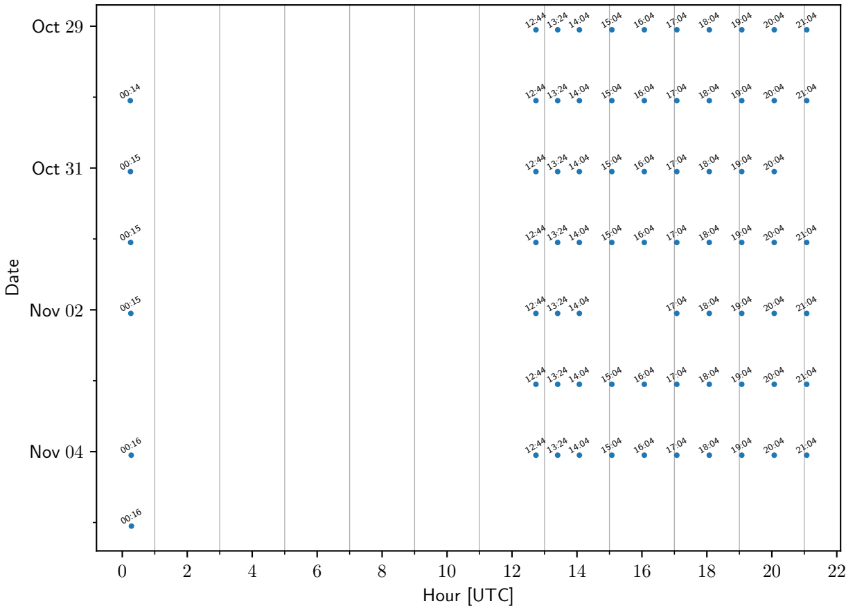
TEMPO sample times: MadisonCT
