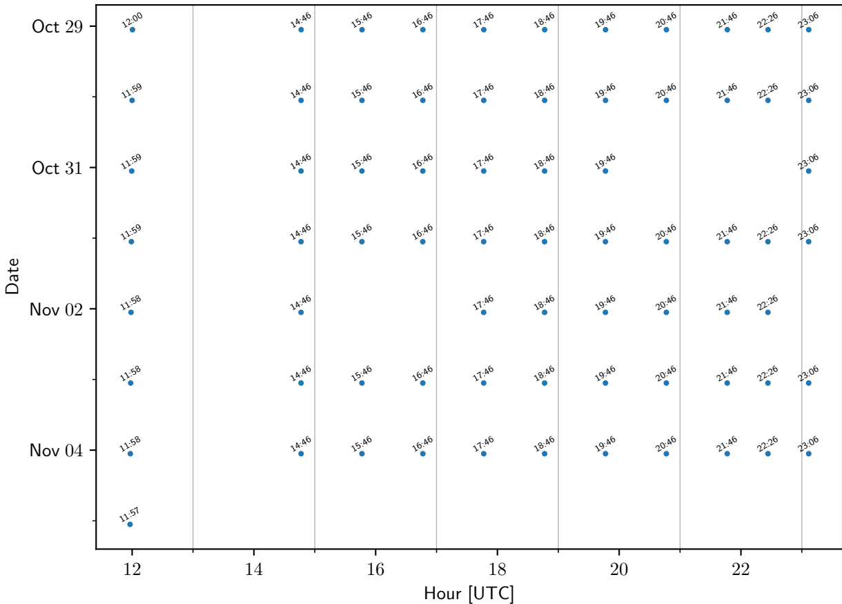
TEMPO sample times: TurlockCA
