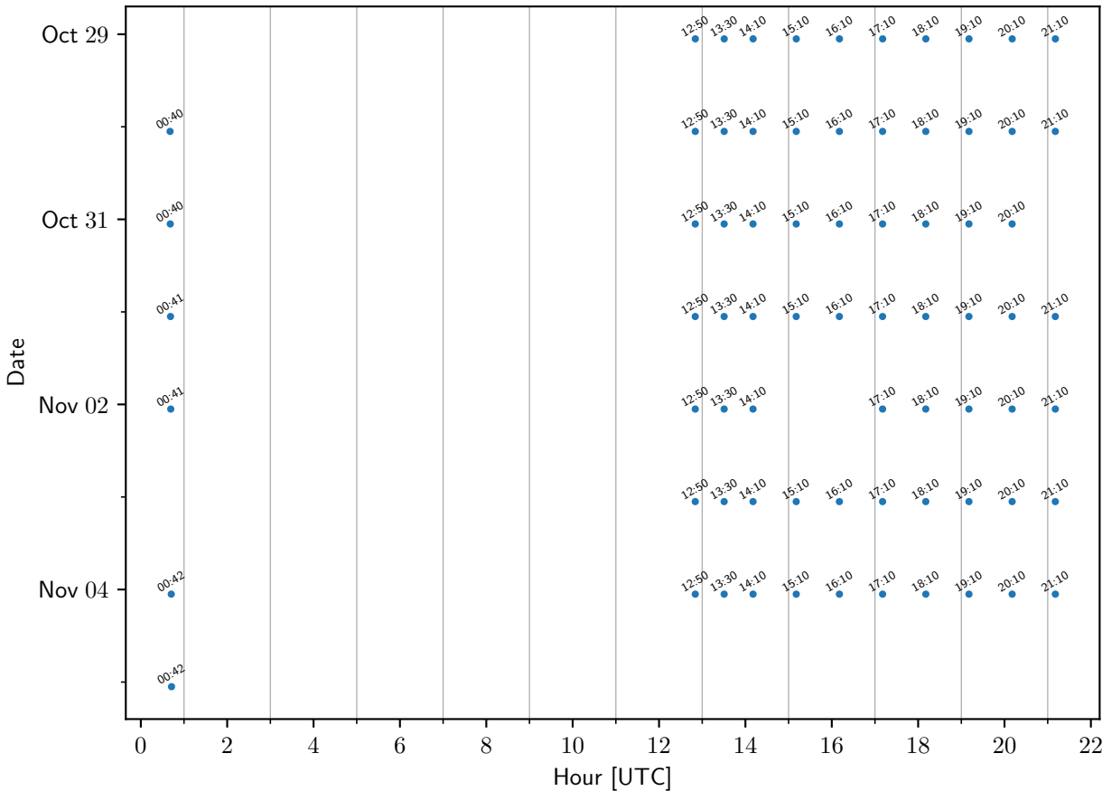
TEMPO sample times: Toronto-CNTower
