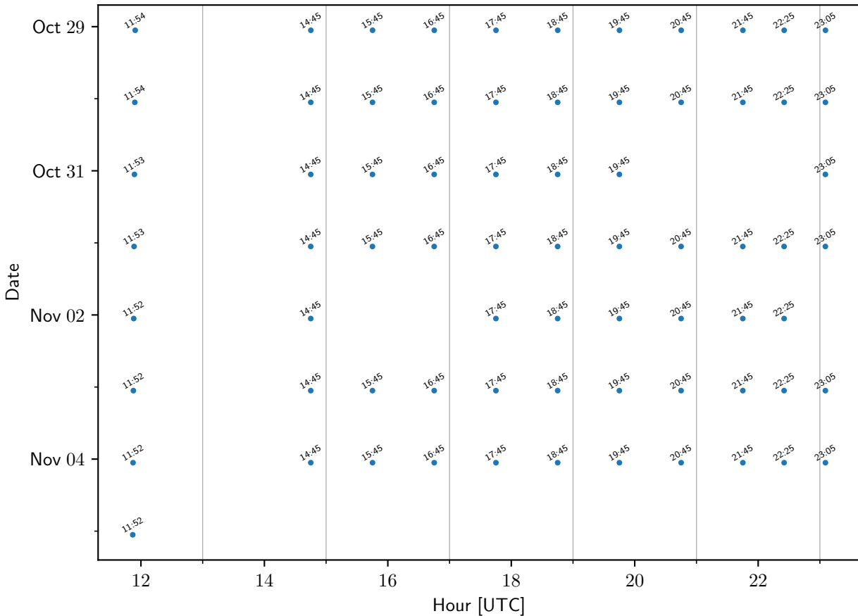
TEMPO sample times: ScaqmdOntarioNR
