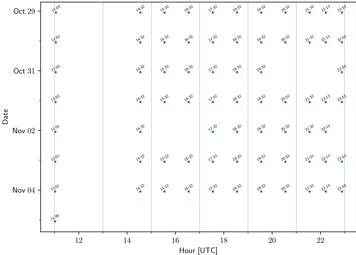
TEMPO sample times: Boulder
