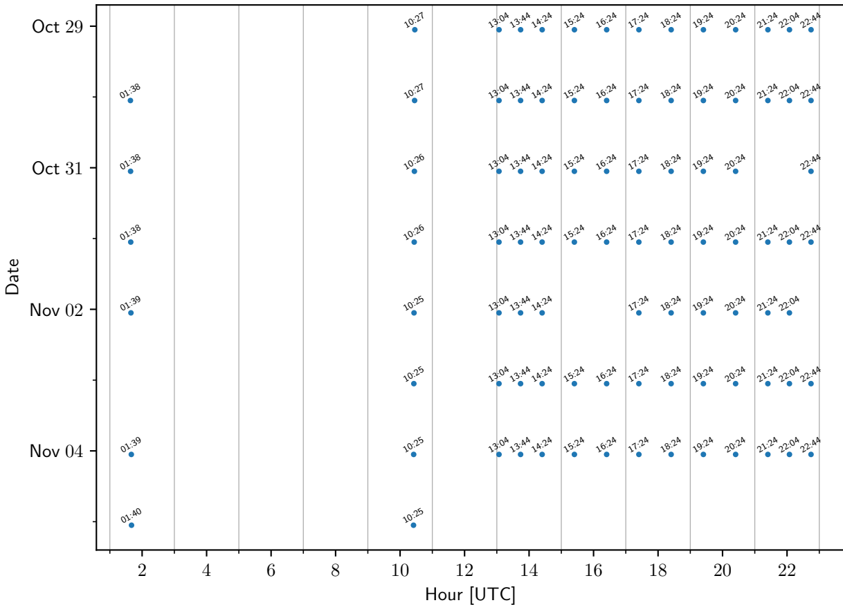
TEMPO sample times: Galveston
