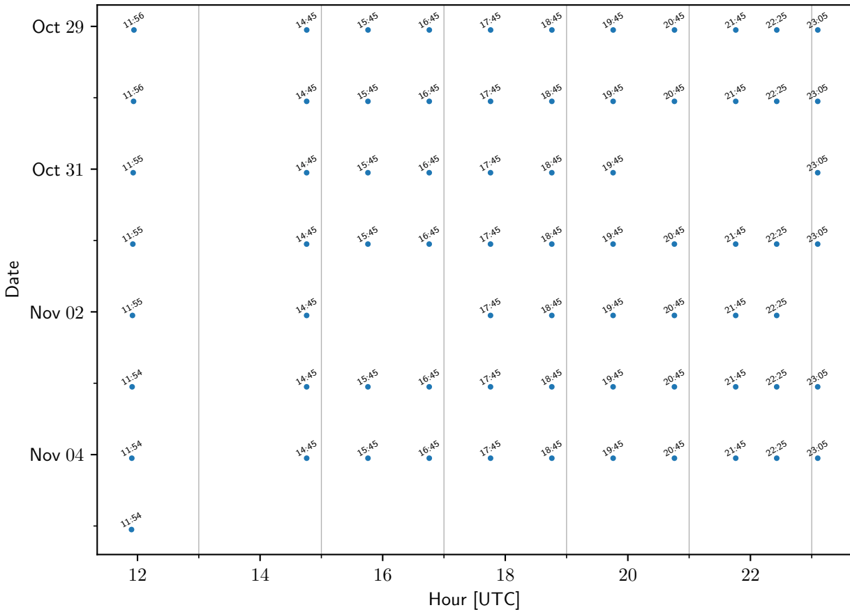
TEMPO sample times: staqs-PASADENA.JPL
