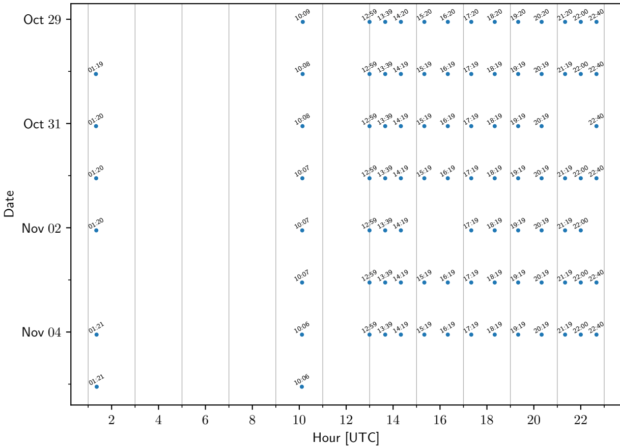
TEMPO sample times: ChauvinLA
