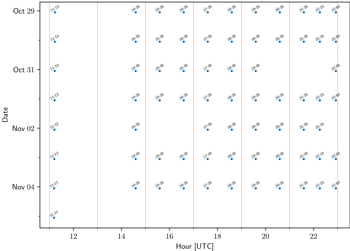
TEMPO sample times: StonyPlain
