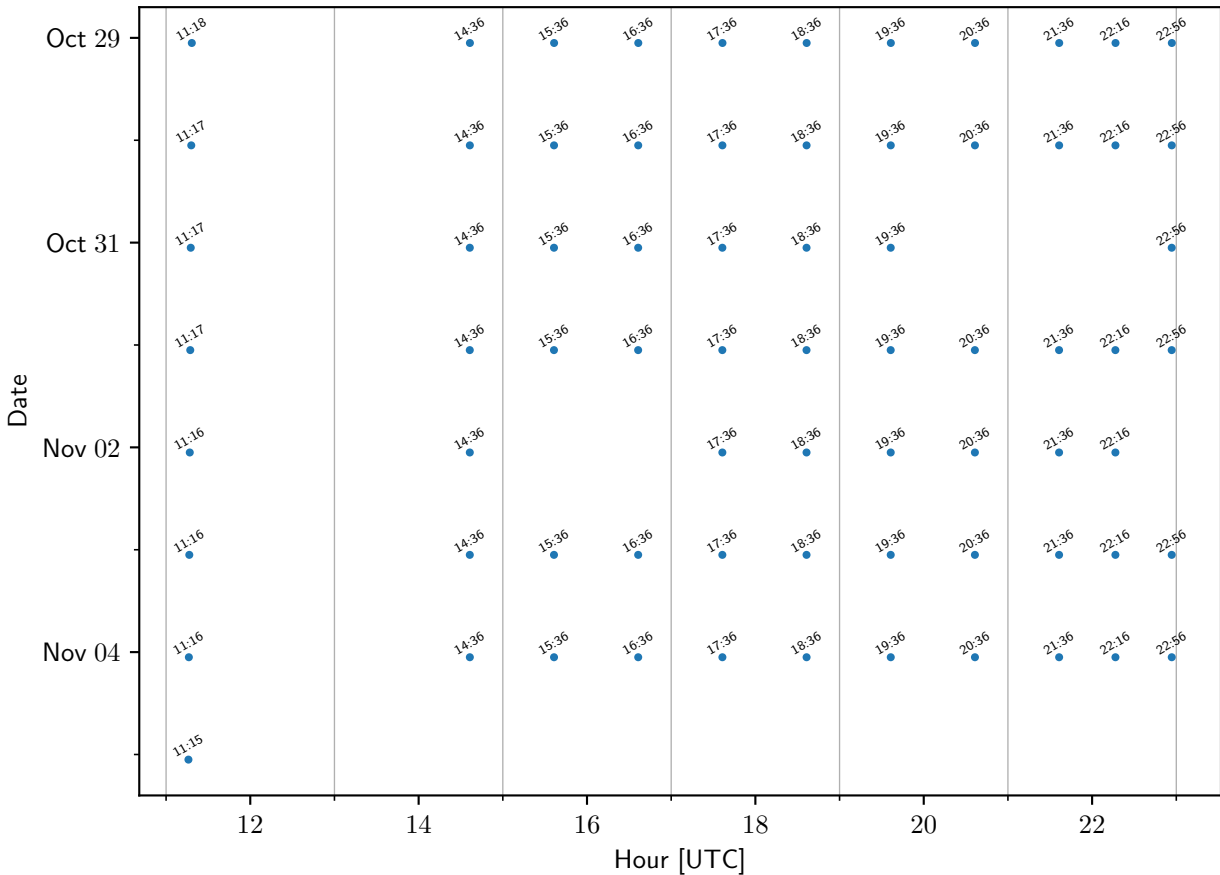
TEMPO sample times: FourCornersNM
