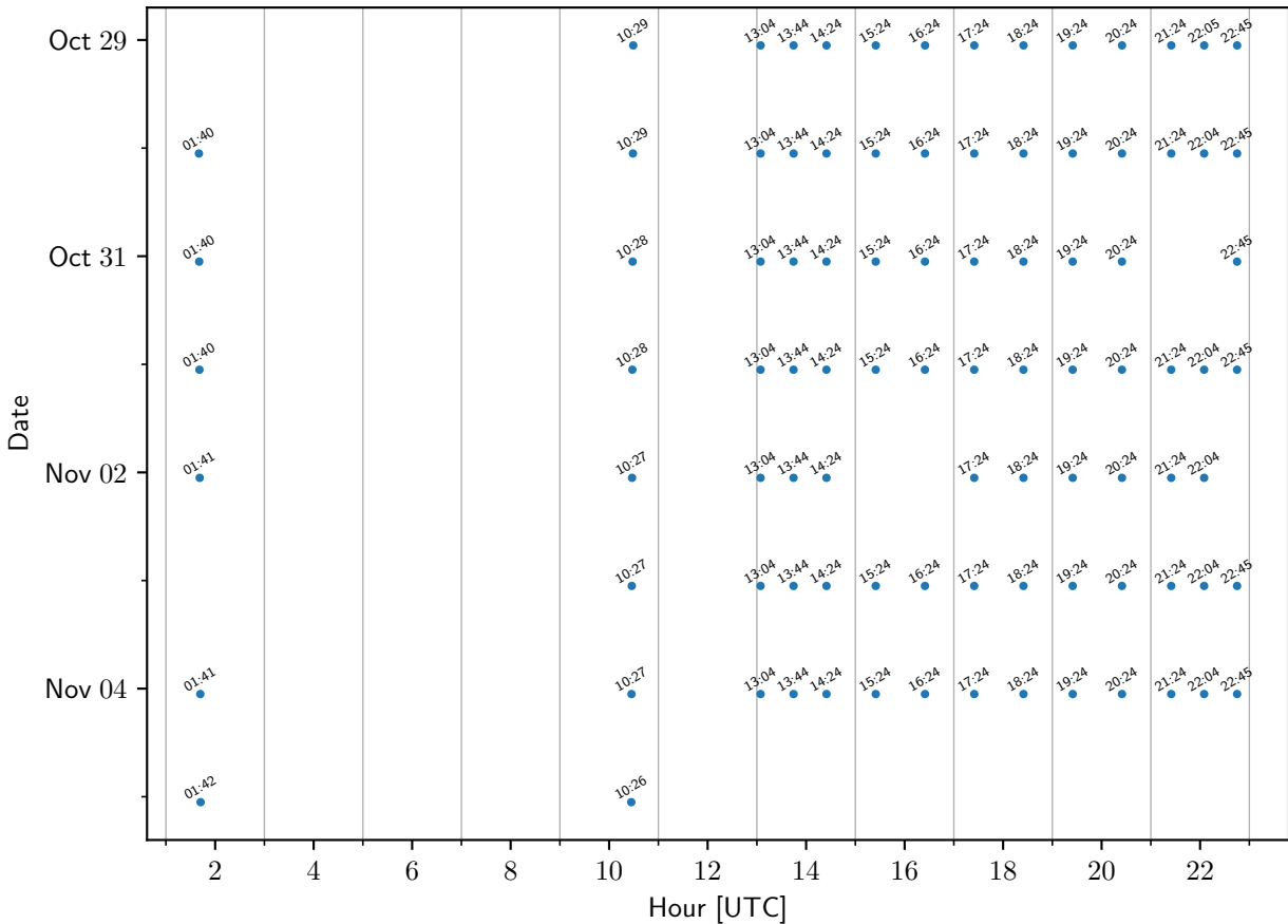
TEMPO sample times: UHMT
