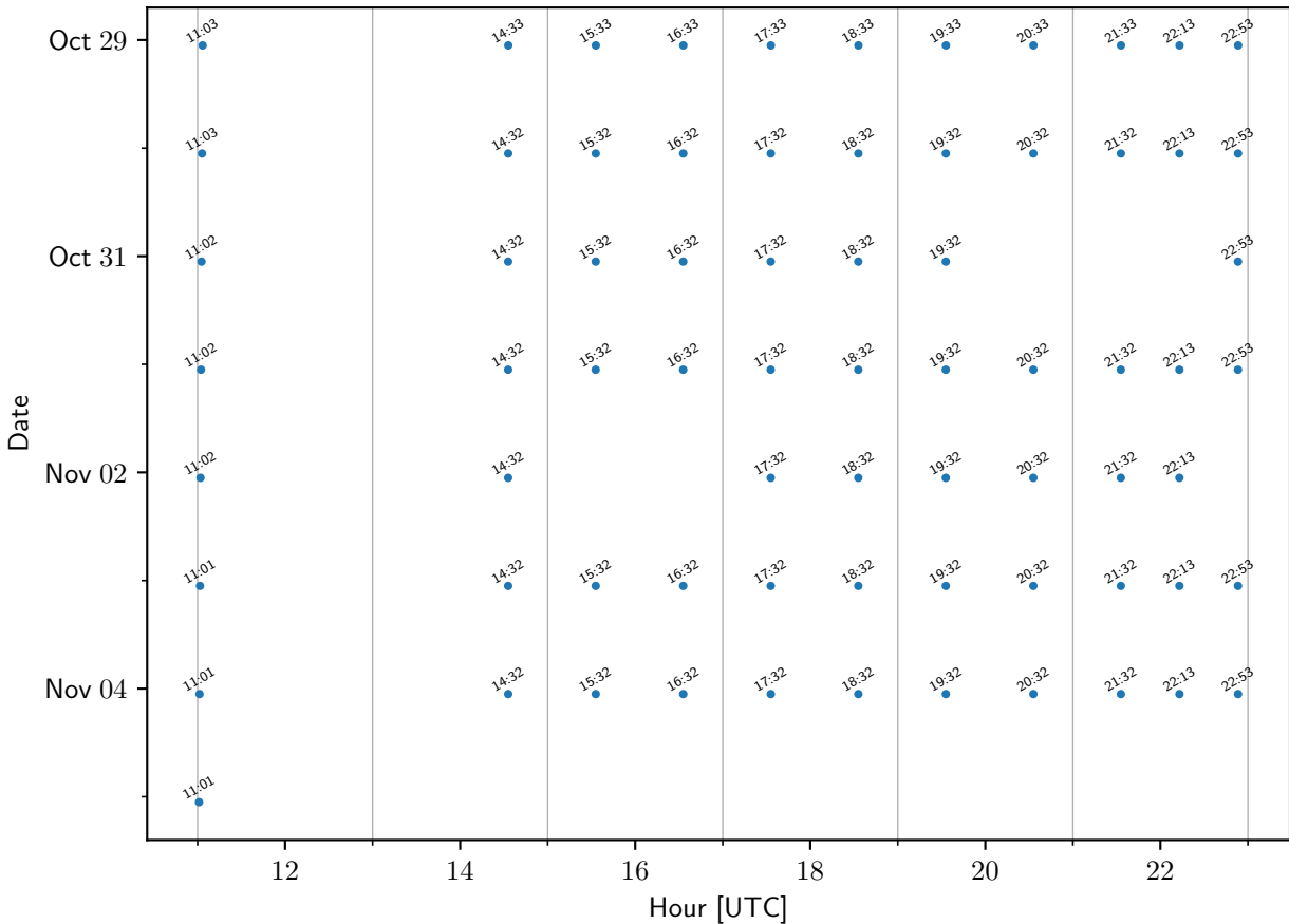
TEMPO sample times: BLD
