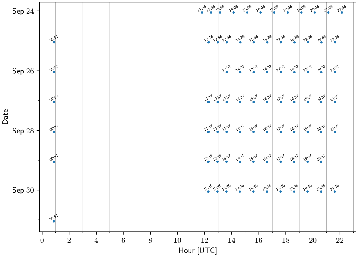
TEMPO sample times: Goose_Bay
