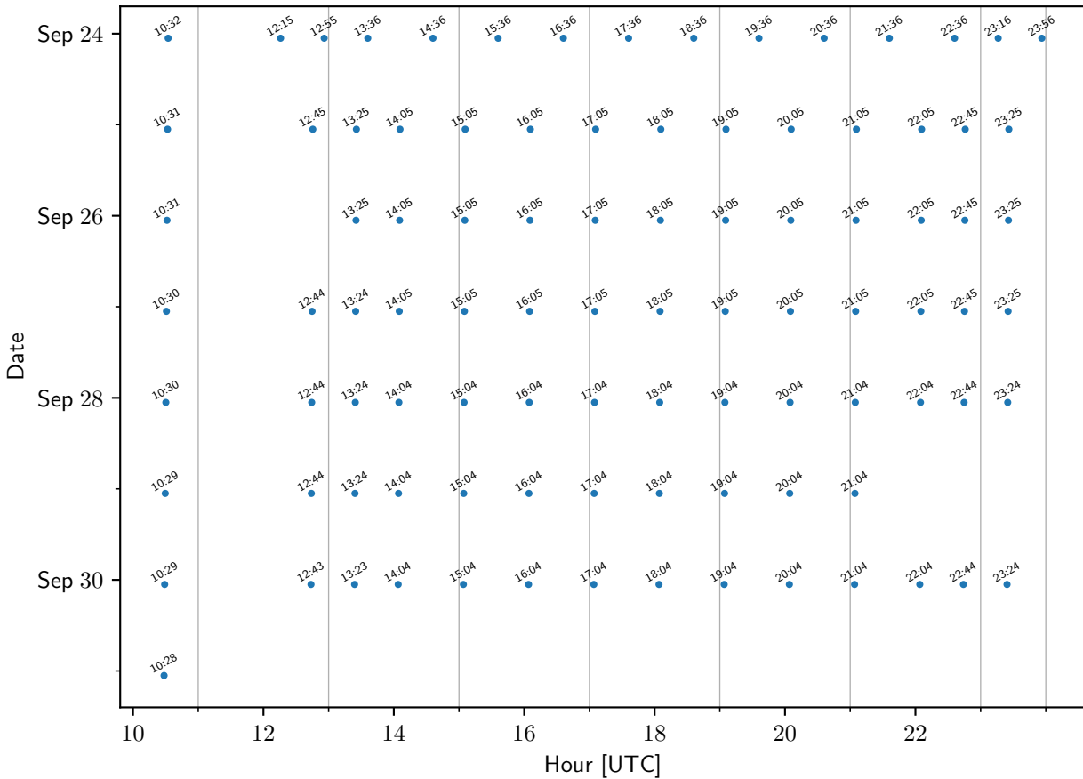
TEMPO sample times: BMK
