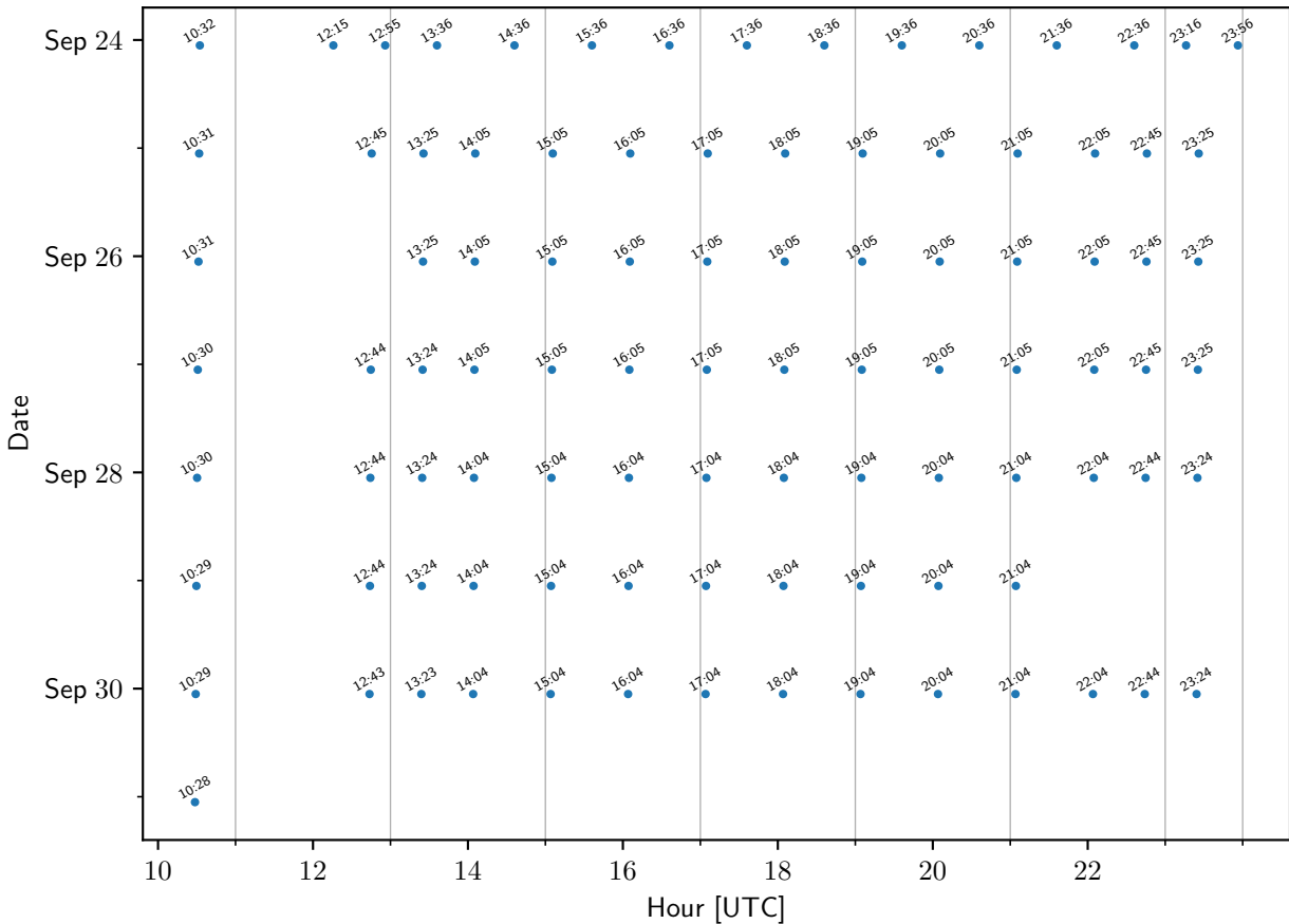
TEMPO sample times: staqs-SanAntonio
