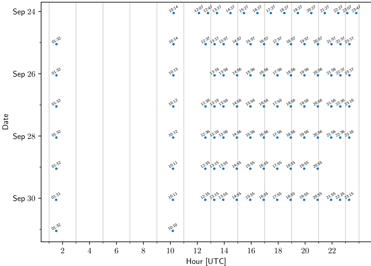
TEMPO sample times: ForestParkM0
