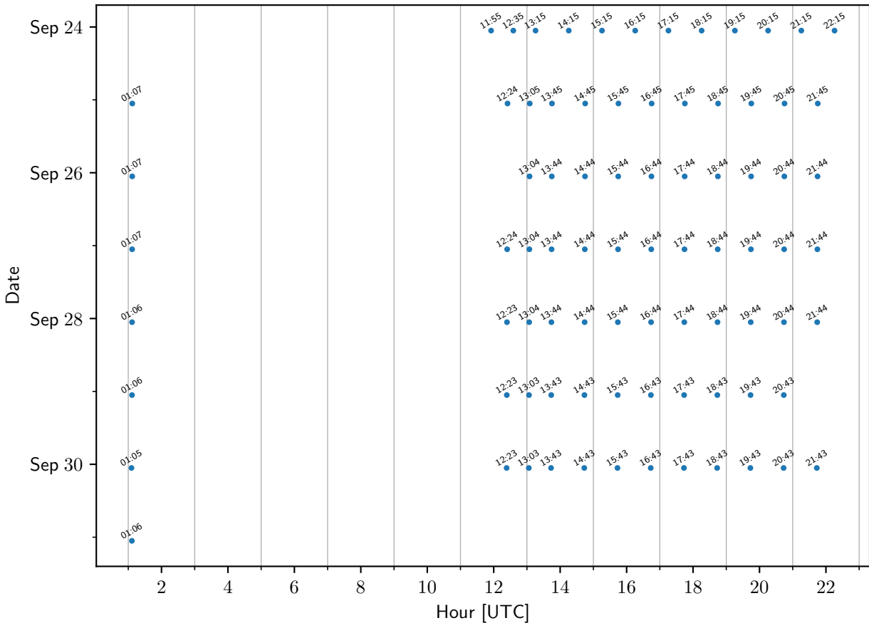
TEMPO sample times: BeltsvilleMD
