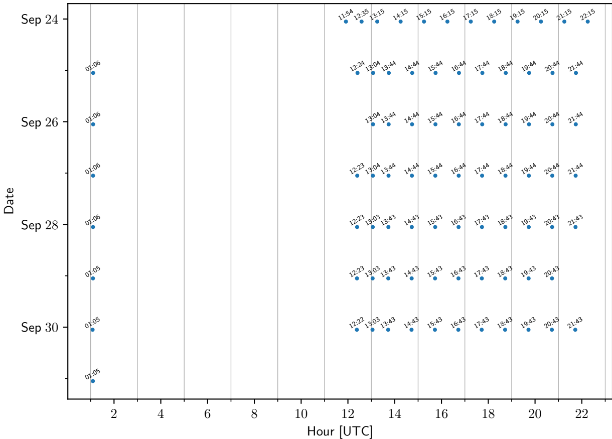
TEMPO sample times: ShipChesapeakeBeachMD
