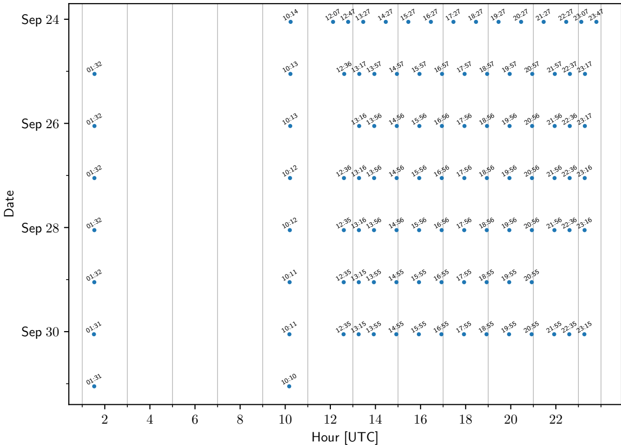
TEMPO sample times: KennerLA
