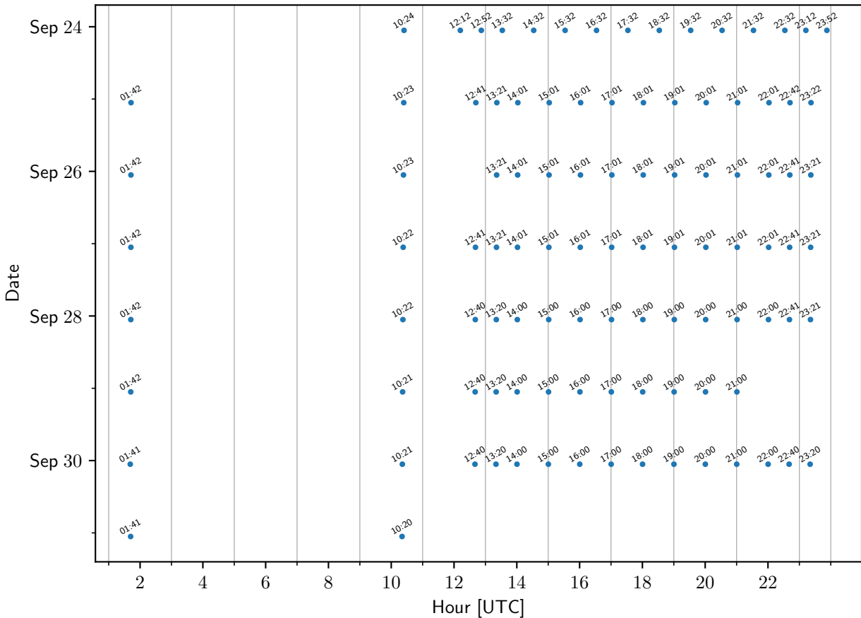
TEMPO sample times: staqs-HoustonGBay
