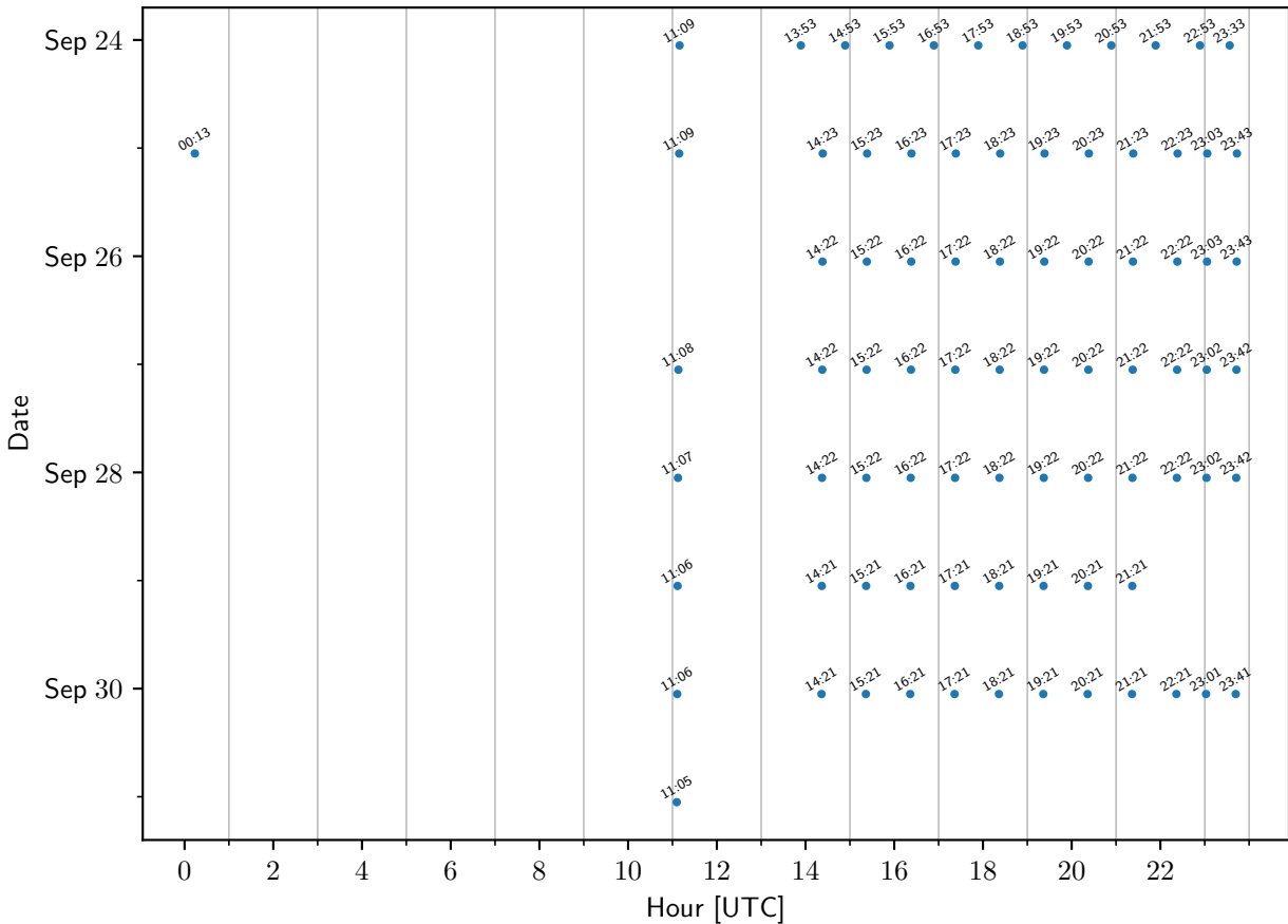
TEMPO sample times: ScaqmdLAMainStreet
