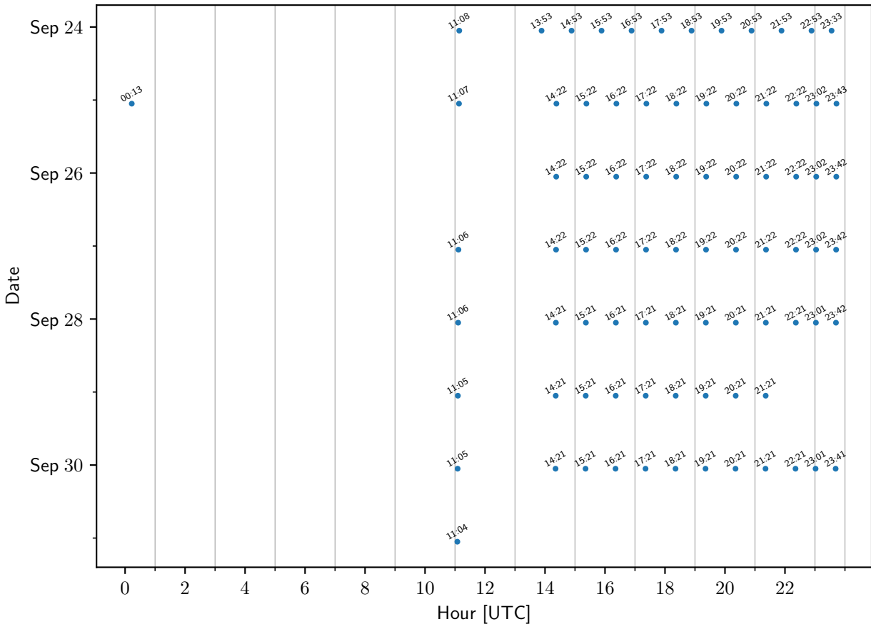
TEMPO sample times: WrightwoodCA
