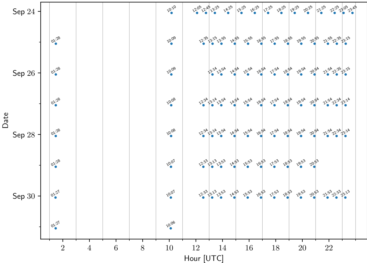
TEMPO sample times: GraftonWI
