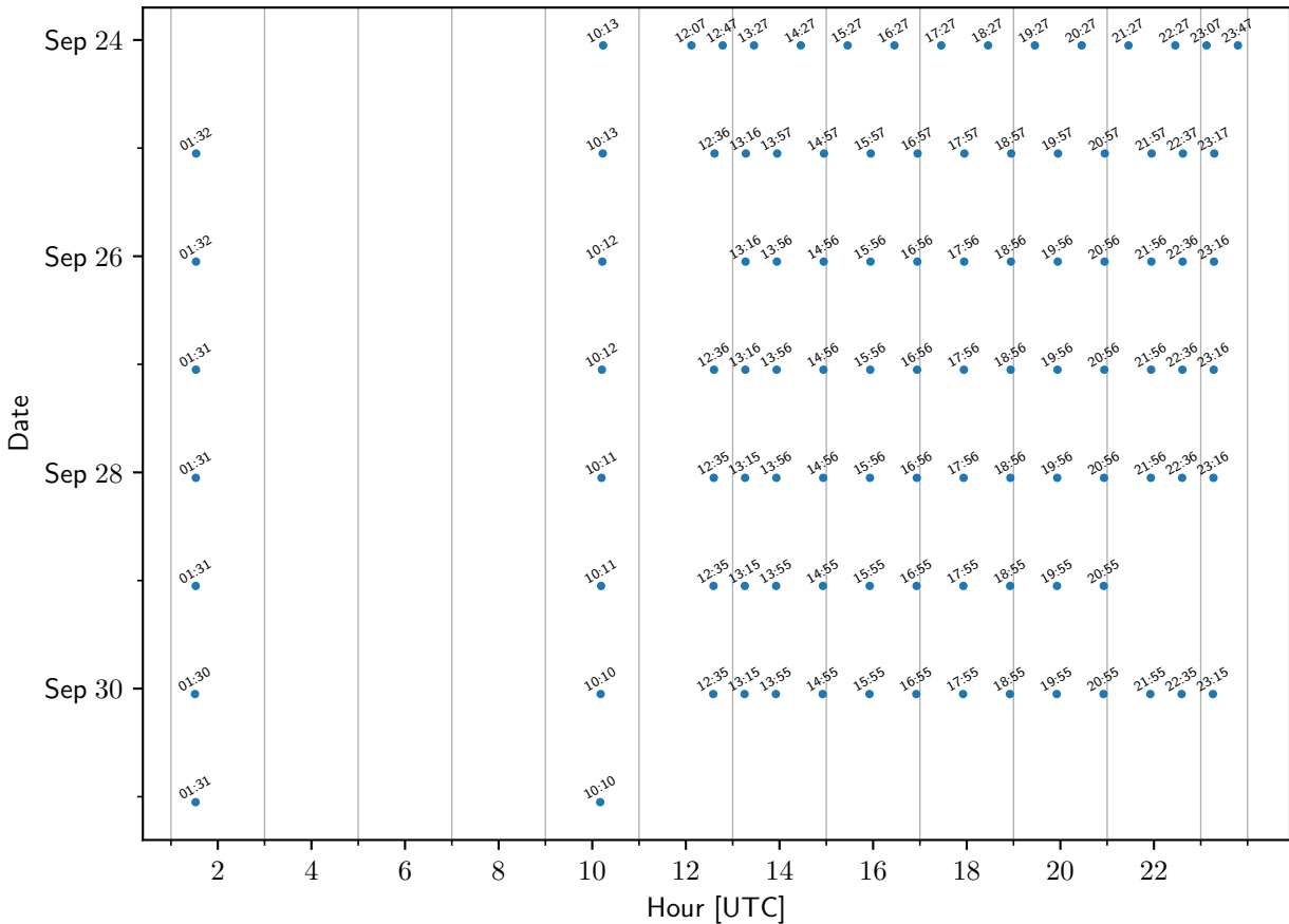
TEMPO sample times: NewOrleansLA-XULA
