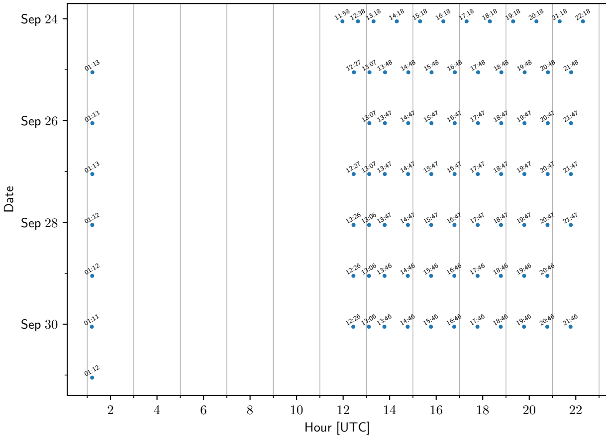
TEMPO sample times: Toronto-Scarborough
