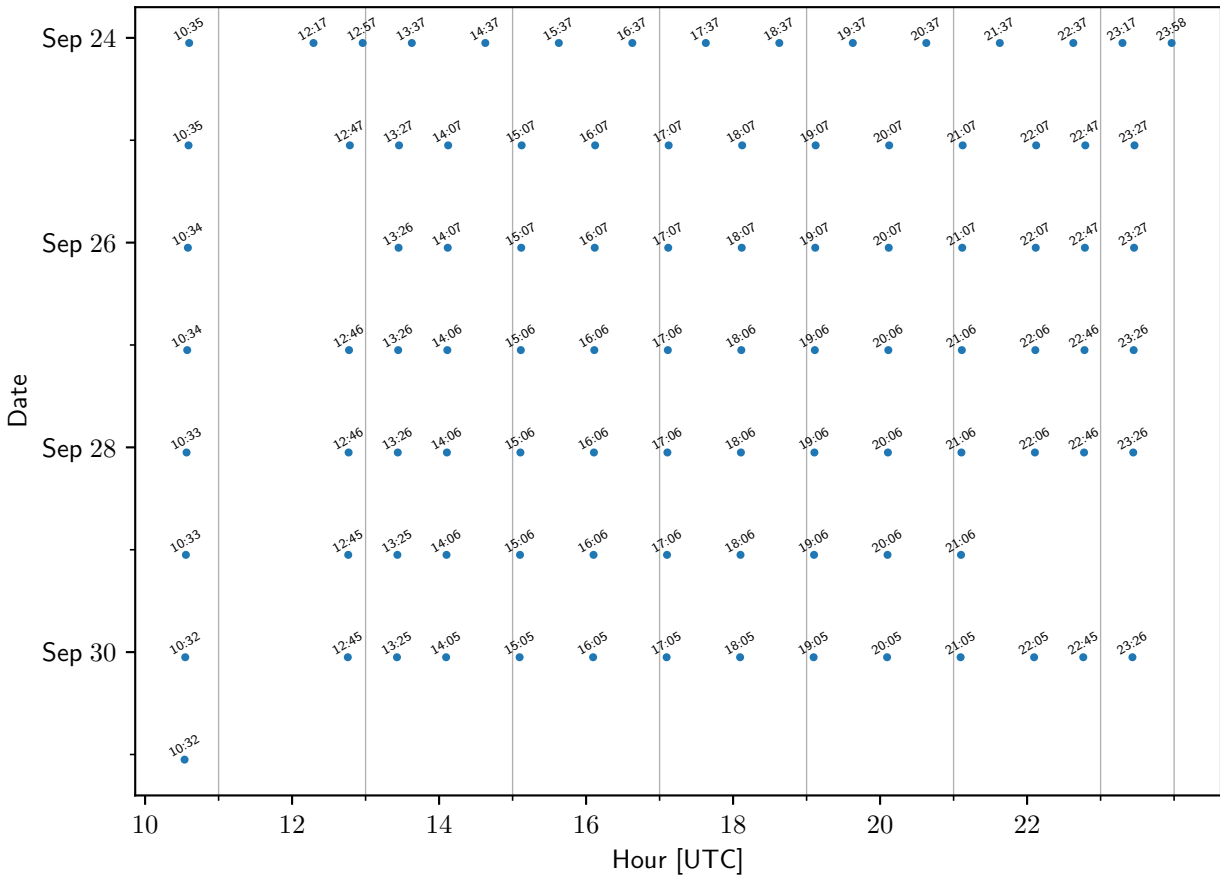
TEMPO sample times: Tula
