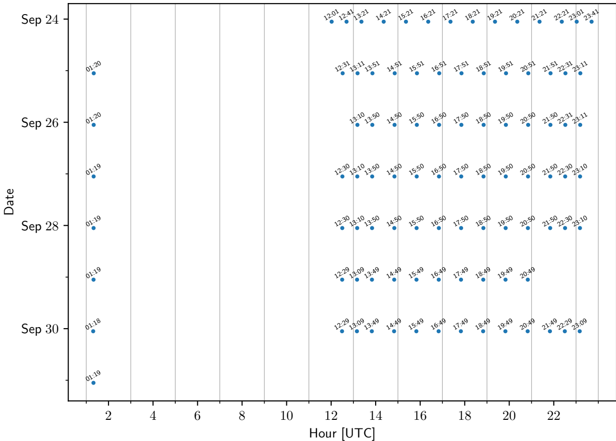
TEMPO sample times: AtlantaGA-SouthDeKalb
