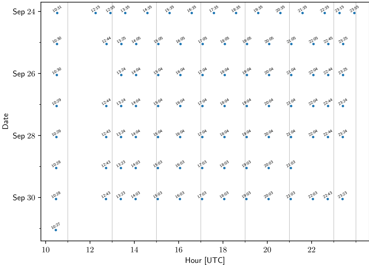
TEMPO sample times: MEX
