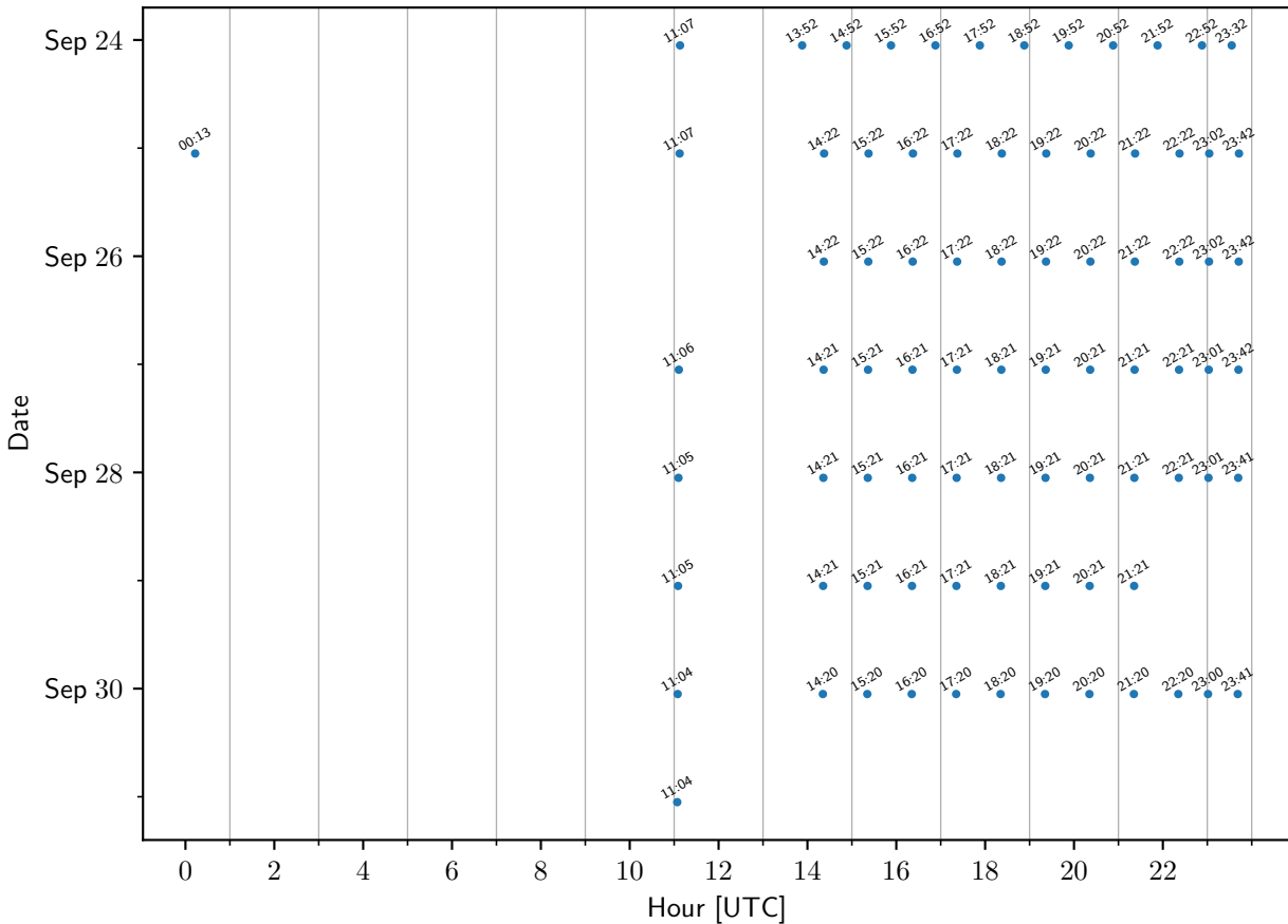
TEMPO sample times: staqs-SAN.BERNARDINO.CALSTATE
