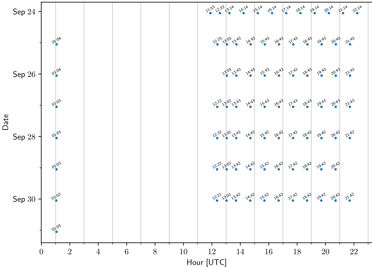
TEMPO sample times: BristolPA
