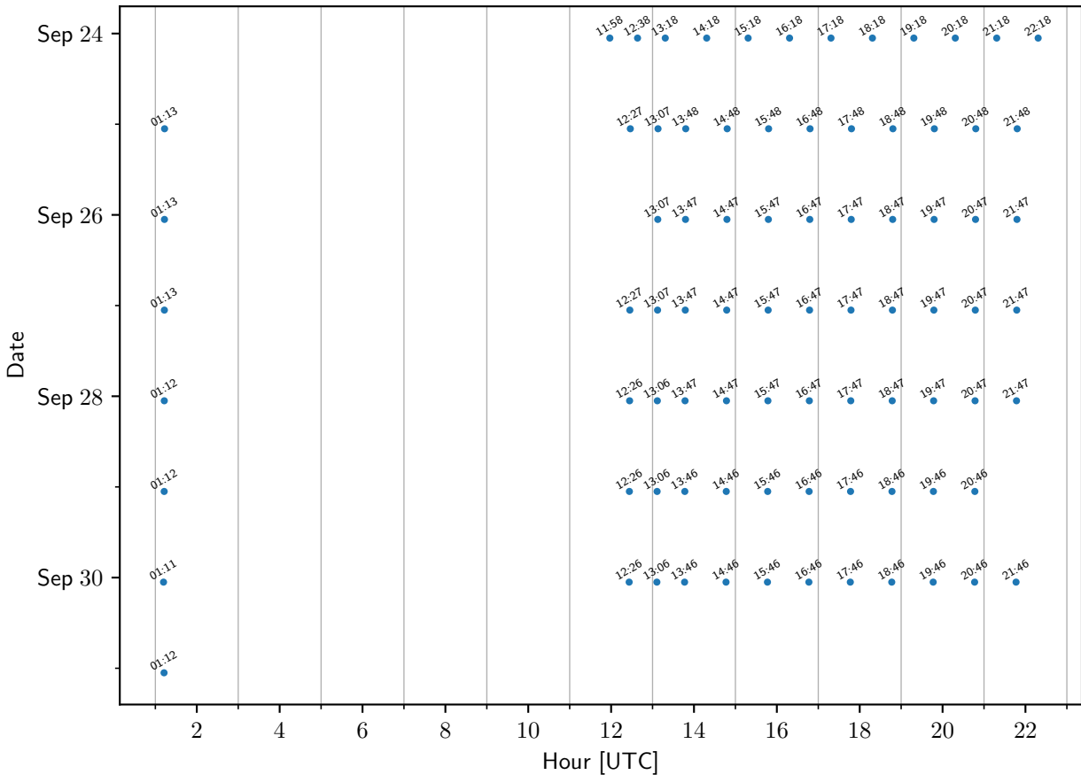
TEMPO sample times: LabVirginiaTech
