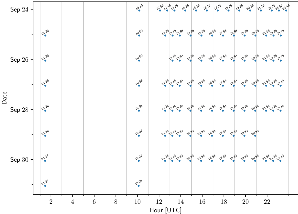
TEMPO sample times: MilwaukeeSER
