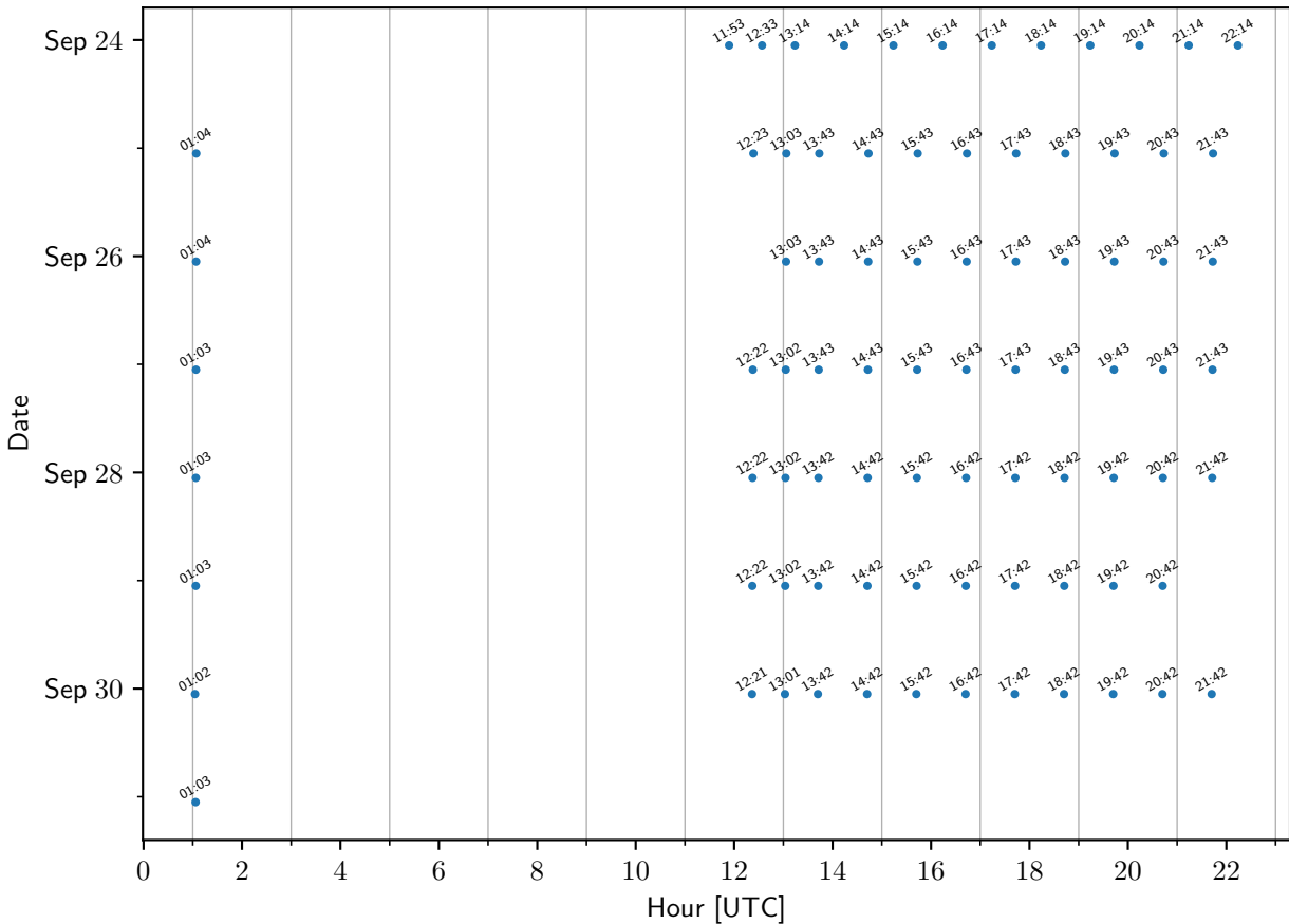
TEMPO sample times: WAI
