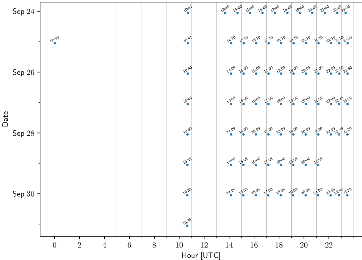
TEMPO sample times: FortMcKay
