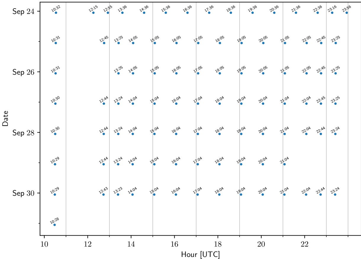
TEMPO sample times: FortYatesND
