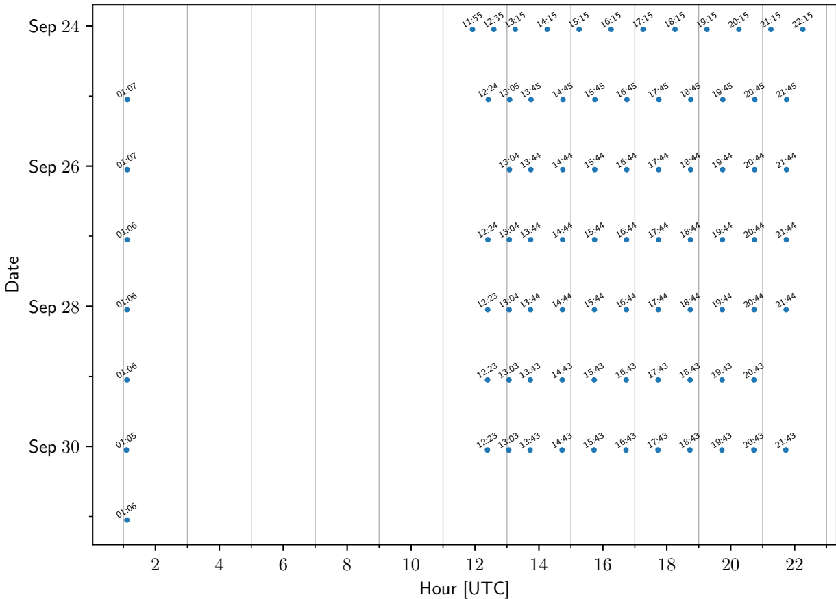
TEMPO sample times: CharlesCityVA
