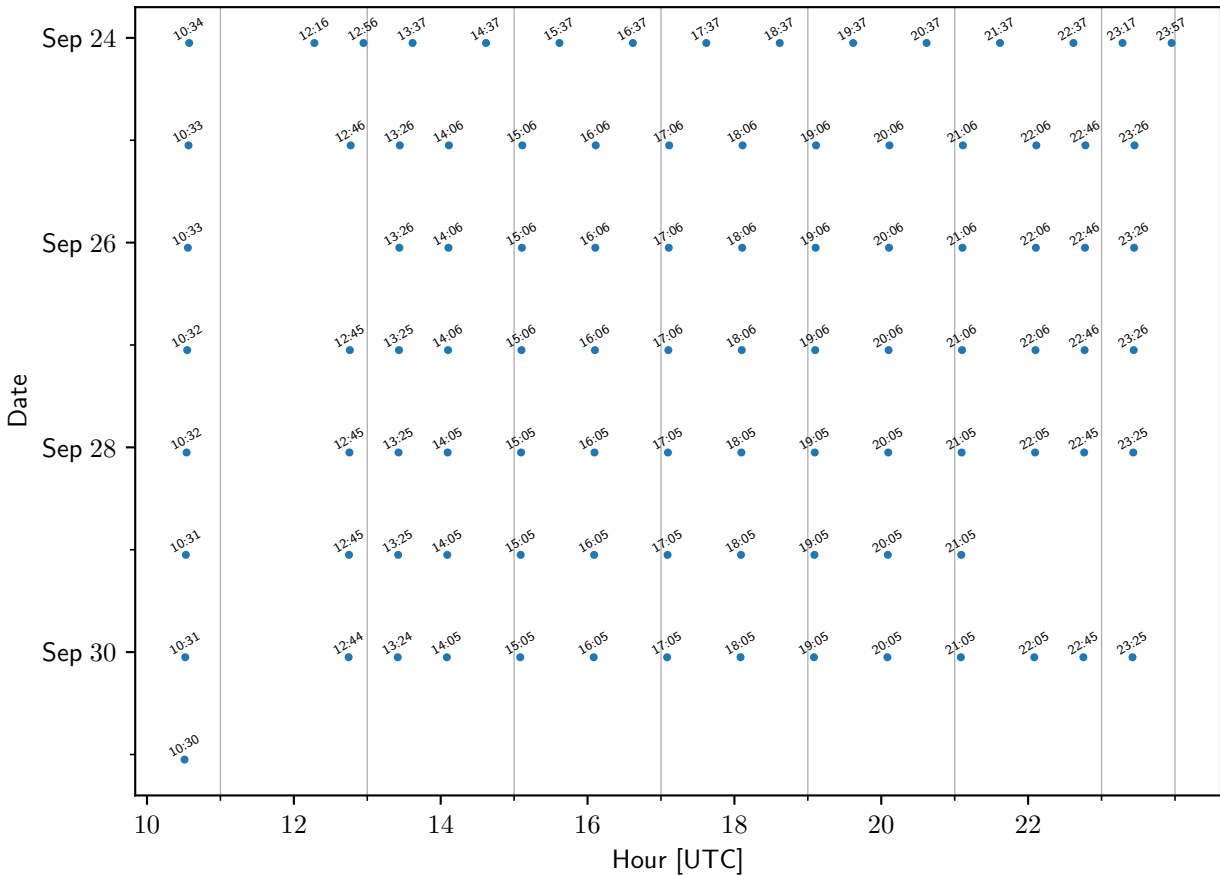
TEMPO sample times: Altzomoni_Atmospheric_Observatory
