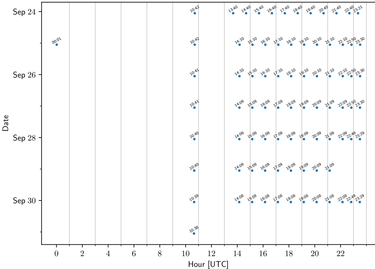
TEMPO sample times: NOAA-CSL
