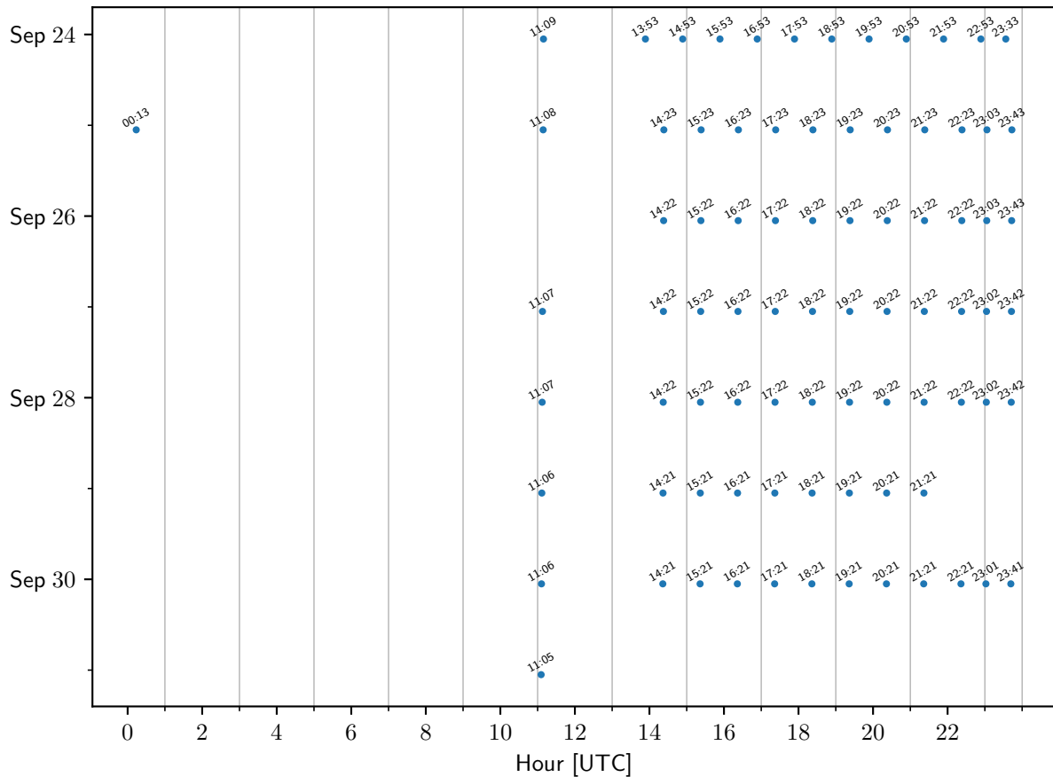
TEMPO sample times: staqs-PASADENA.JPL
