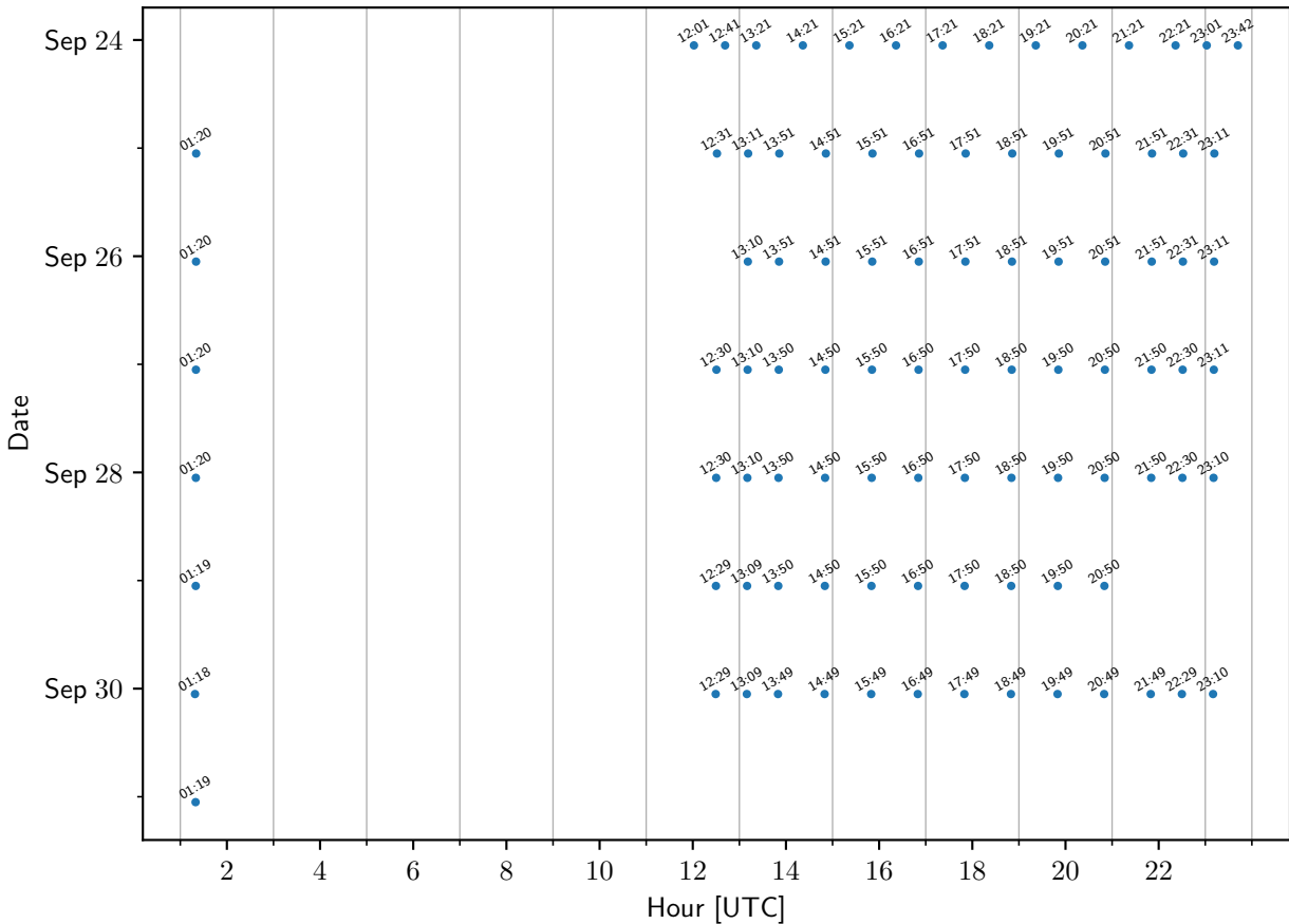
TEMPO sample times: AtlantaATL
