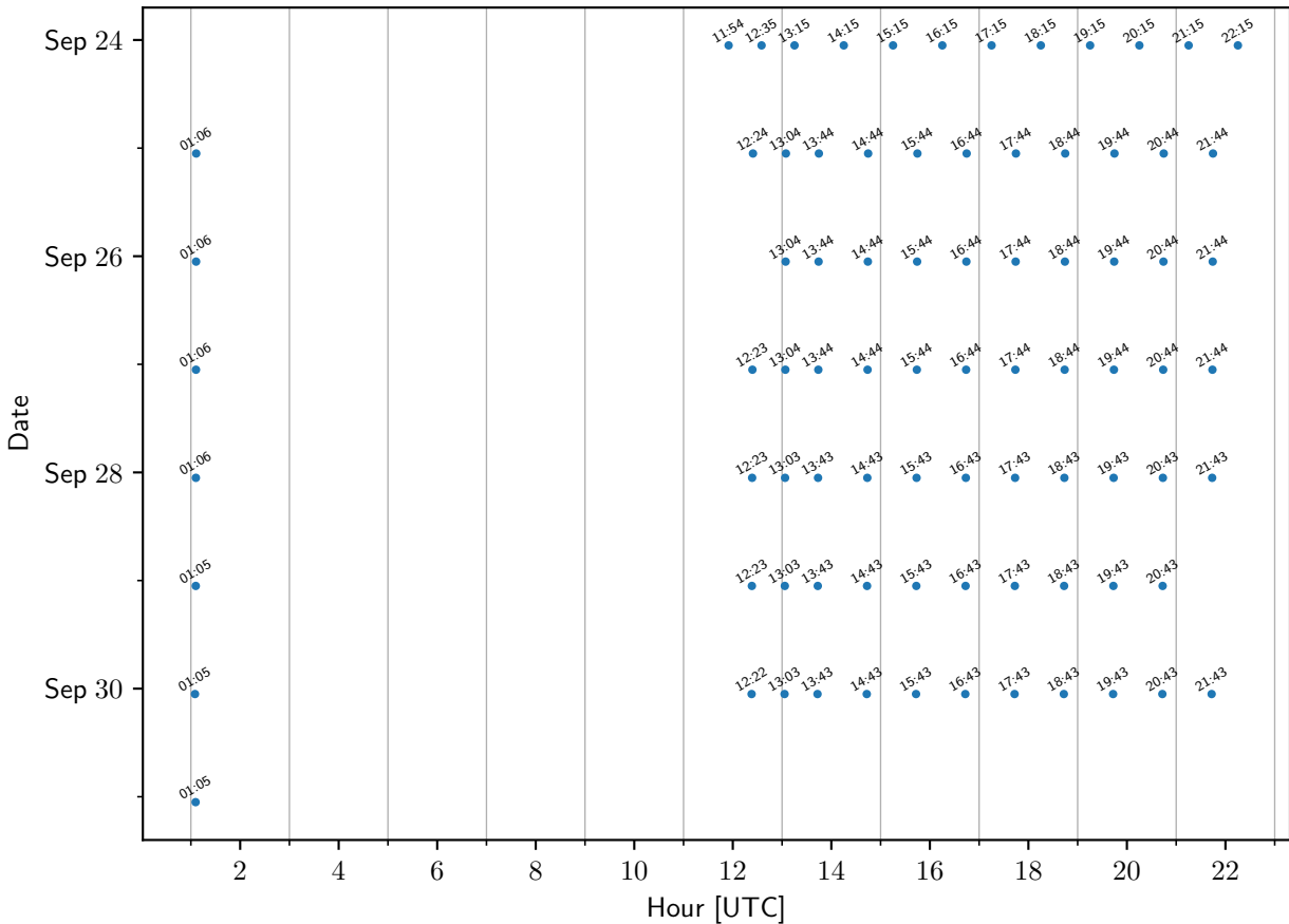
TEMPO sample times: ChesapeakeBay
