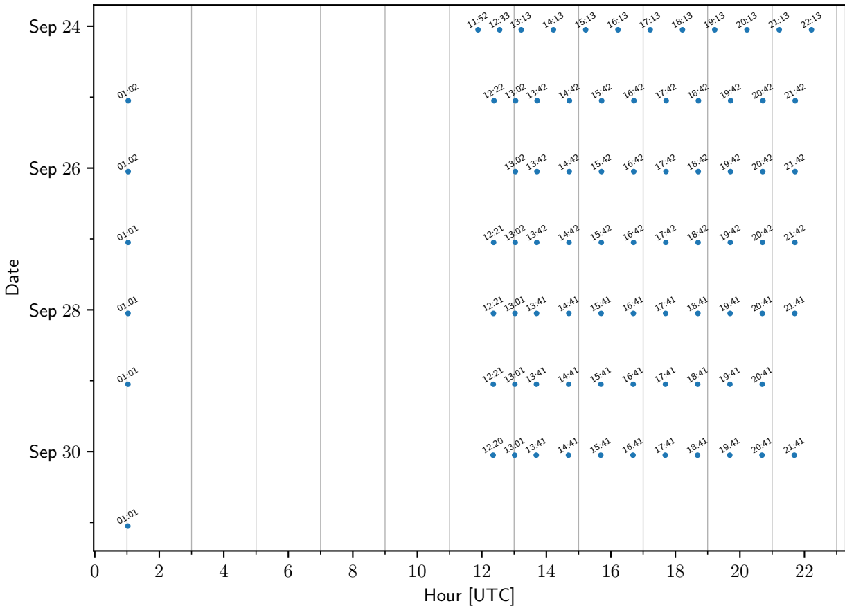
TEMPO sample times: CornwallCT
