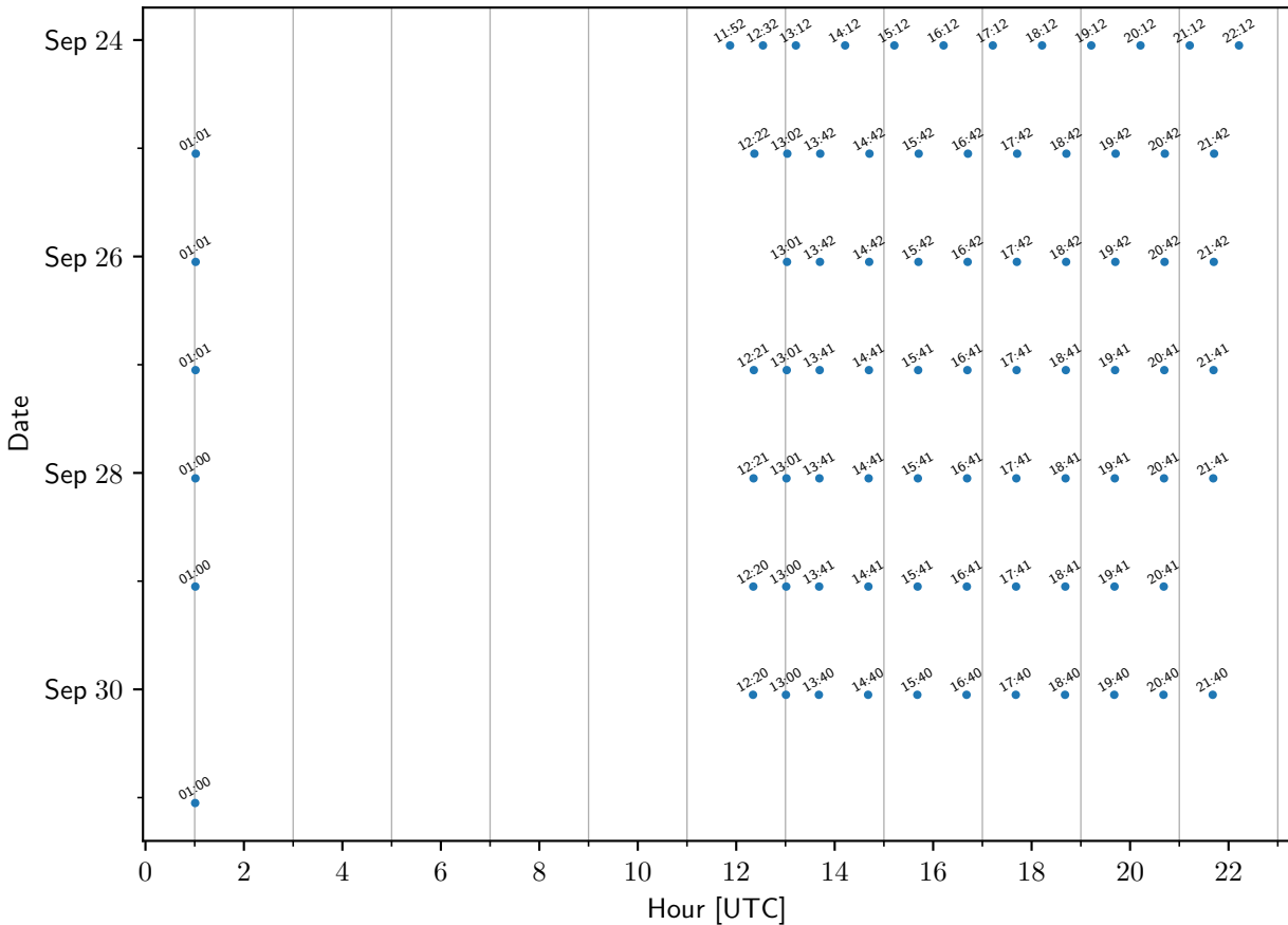
TEMPO sample times: staqs-GUILFORD.YCFS
