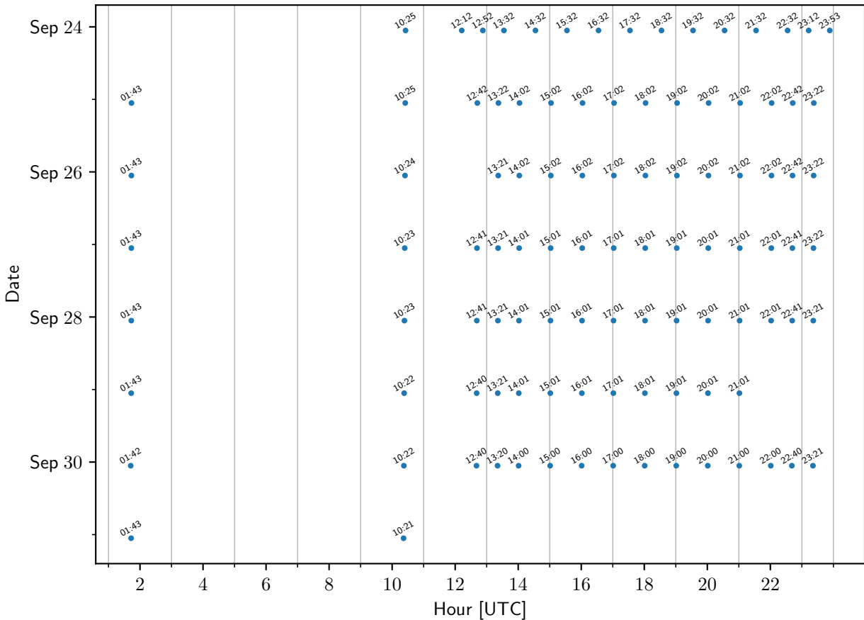
TEMPO sample times: staqs-Houston
