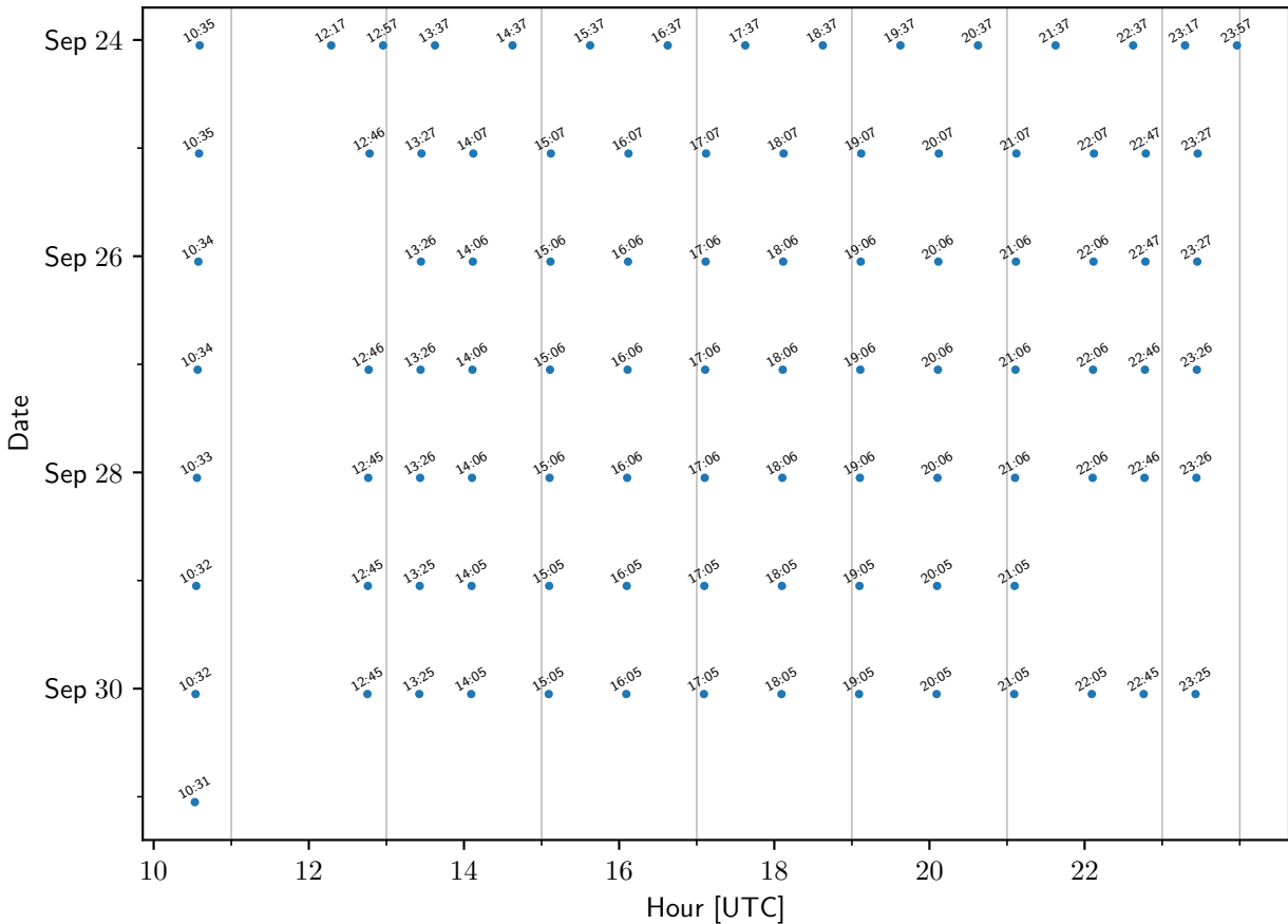
TEMPO sample times: Vallejo
