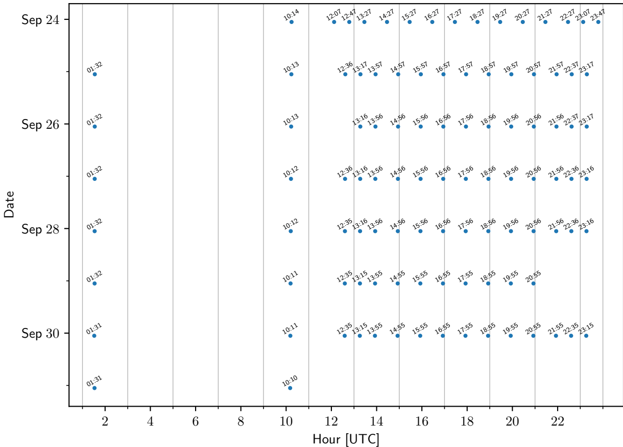
TEMPO sample times: SLU
