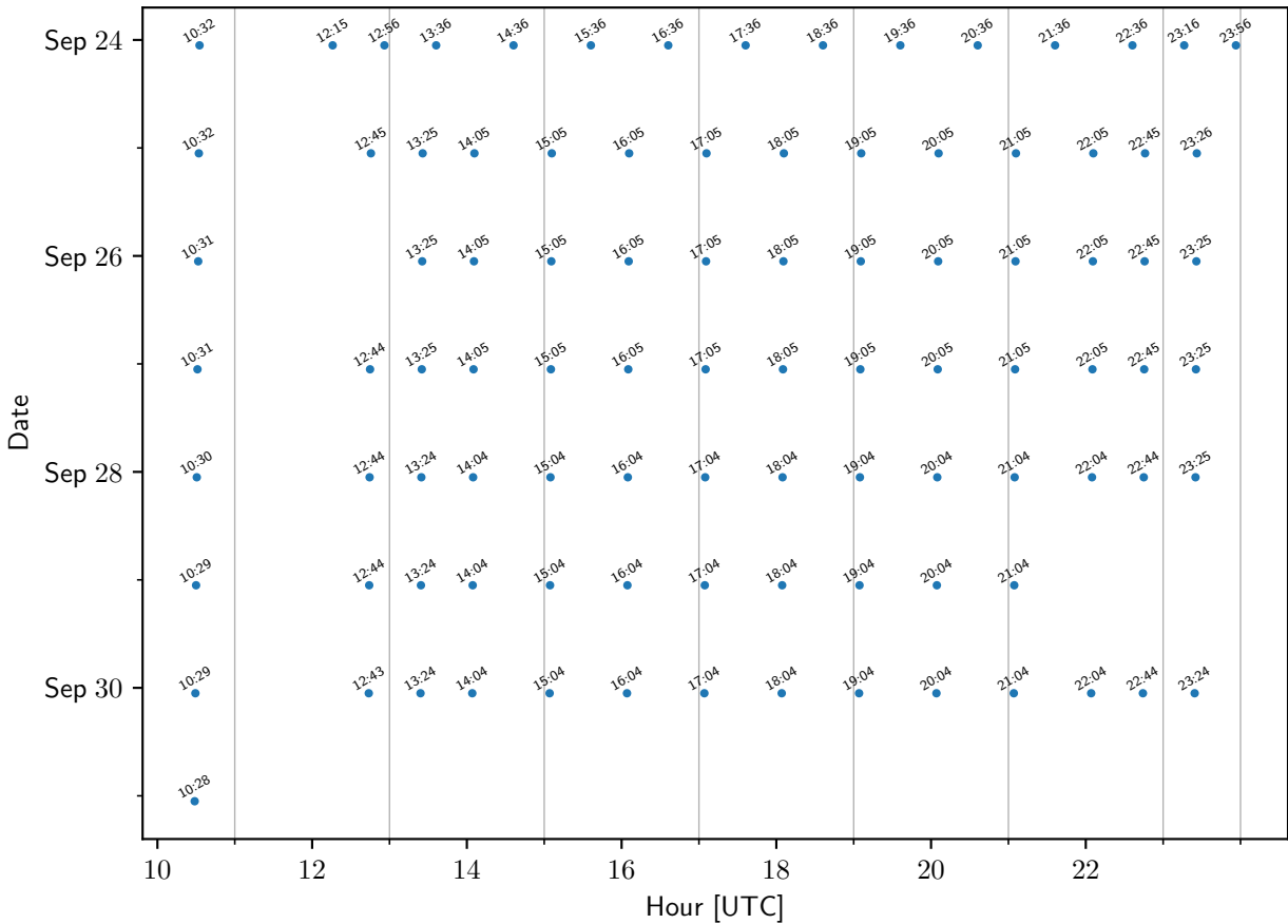
TEMPO sample times: UTSA
