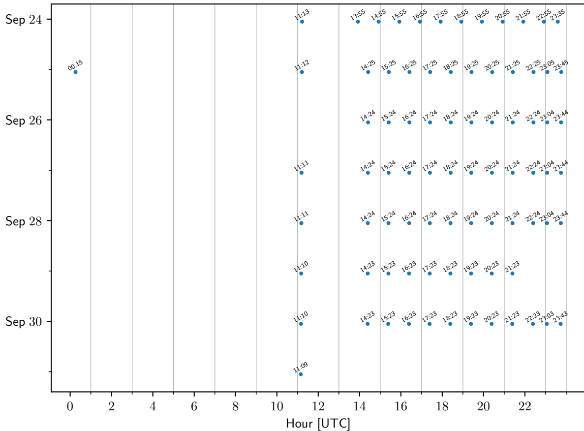
TEMPO sample times: Trinidad_Head
