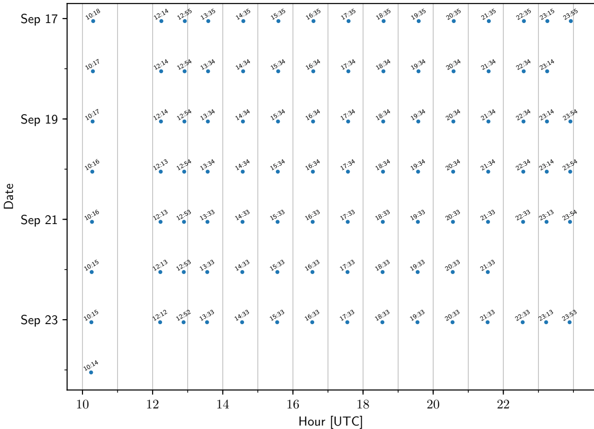
TEMPO sample times: AldineTX
