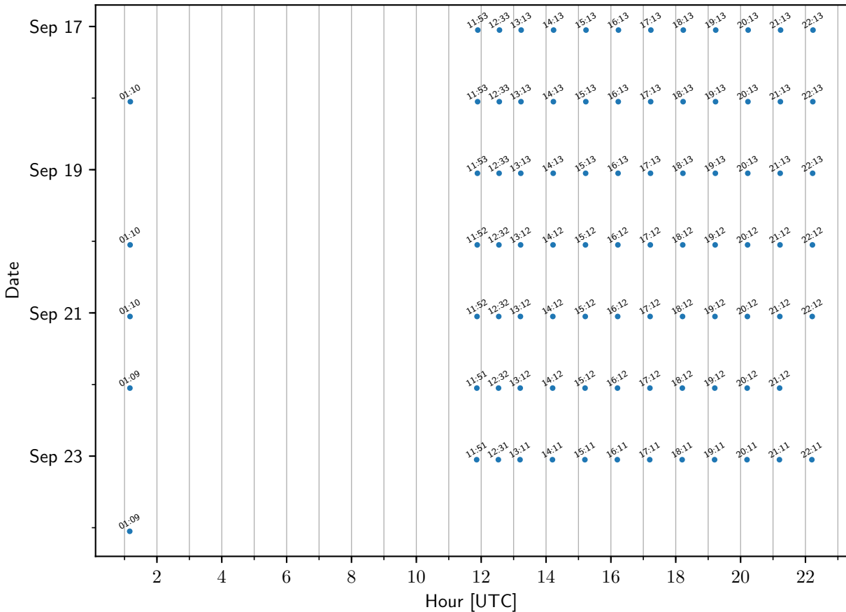
TEMPO sample times: BlueHillMA
