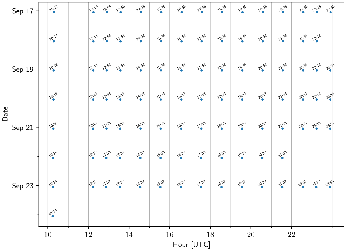
TEMPO sample times: Deerpark
