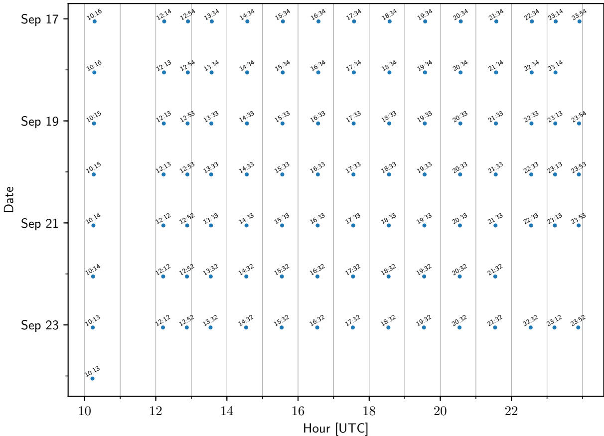
TEMPO sample times: staqs-HoustonGult
