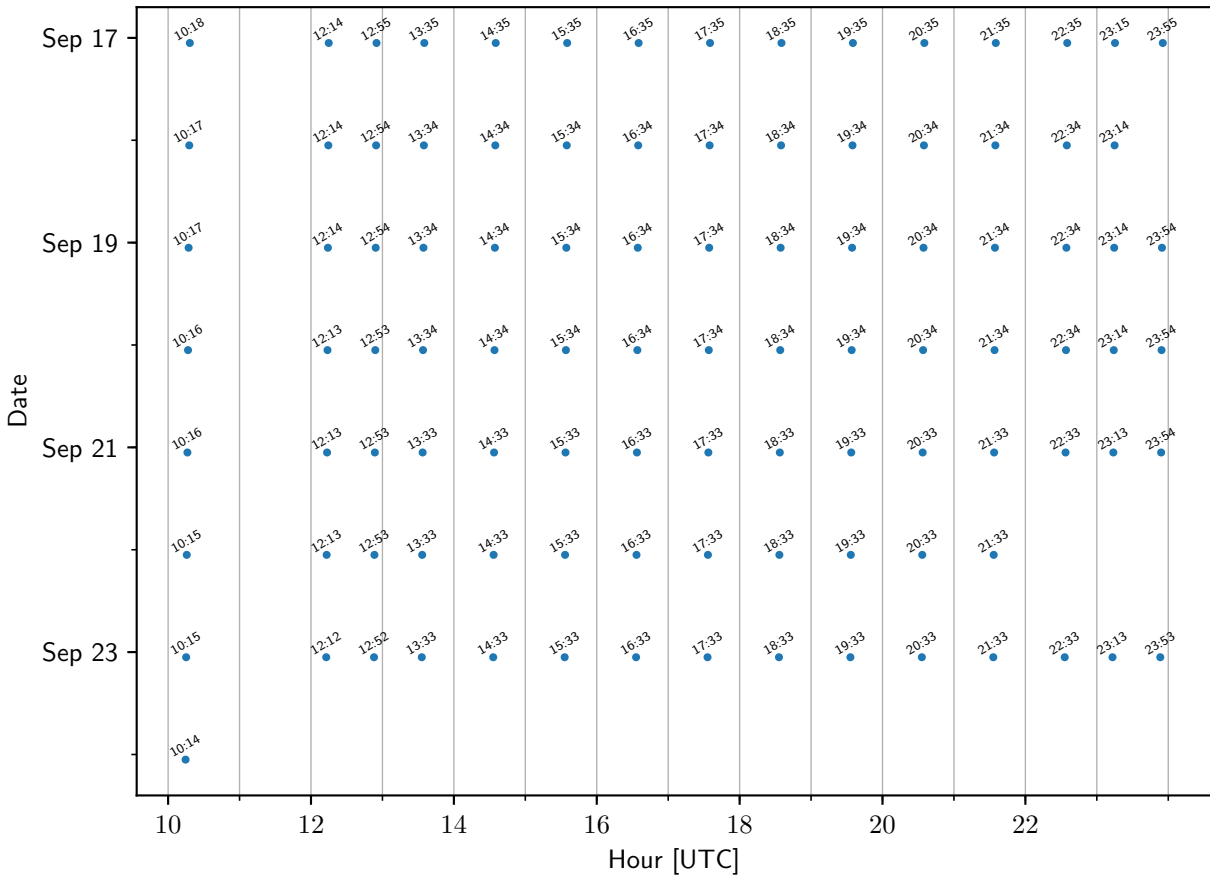
TEMPO sample times: TylerTX
