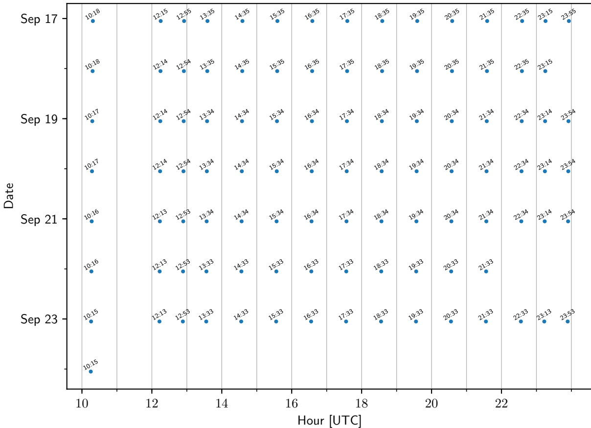
TEMPO sample times: GrandForksND
