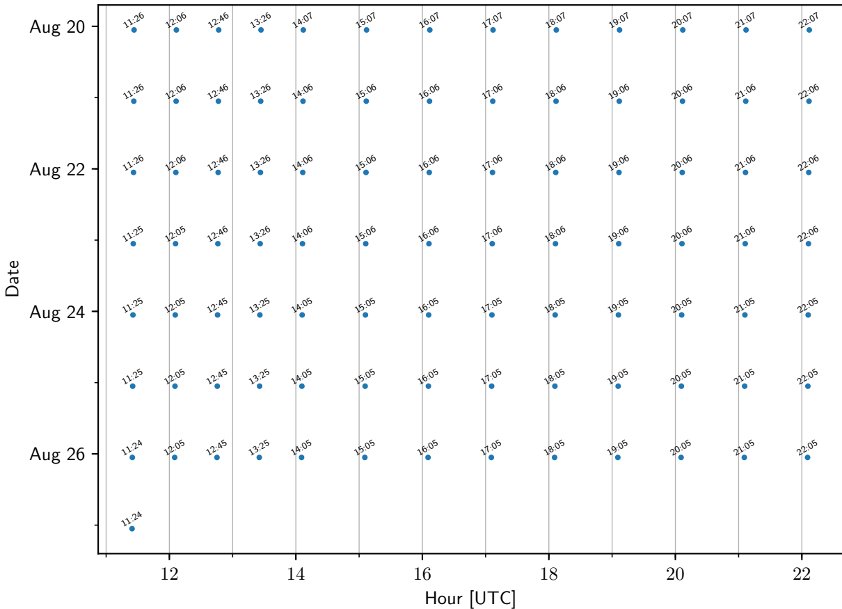
TEMPO sample times: WashingtonDC
