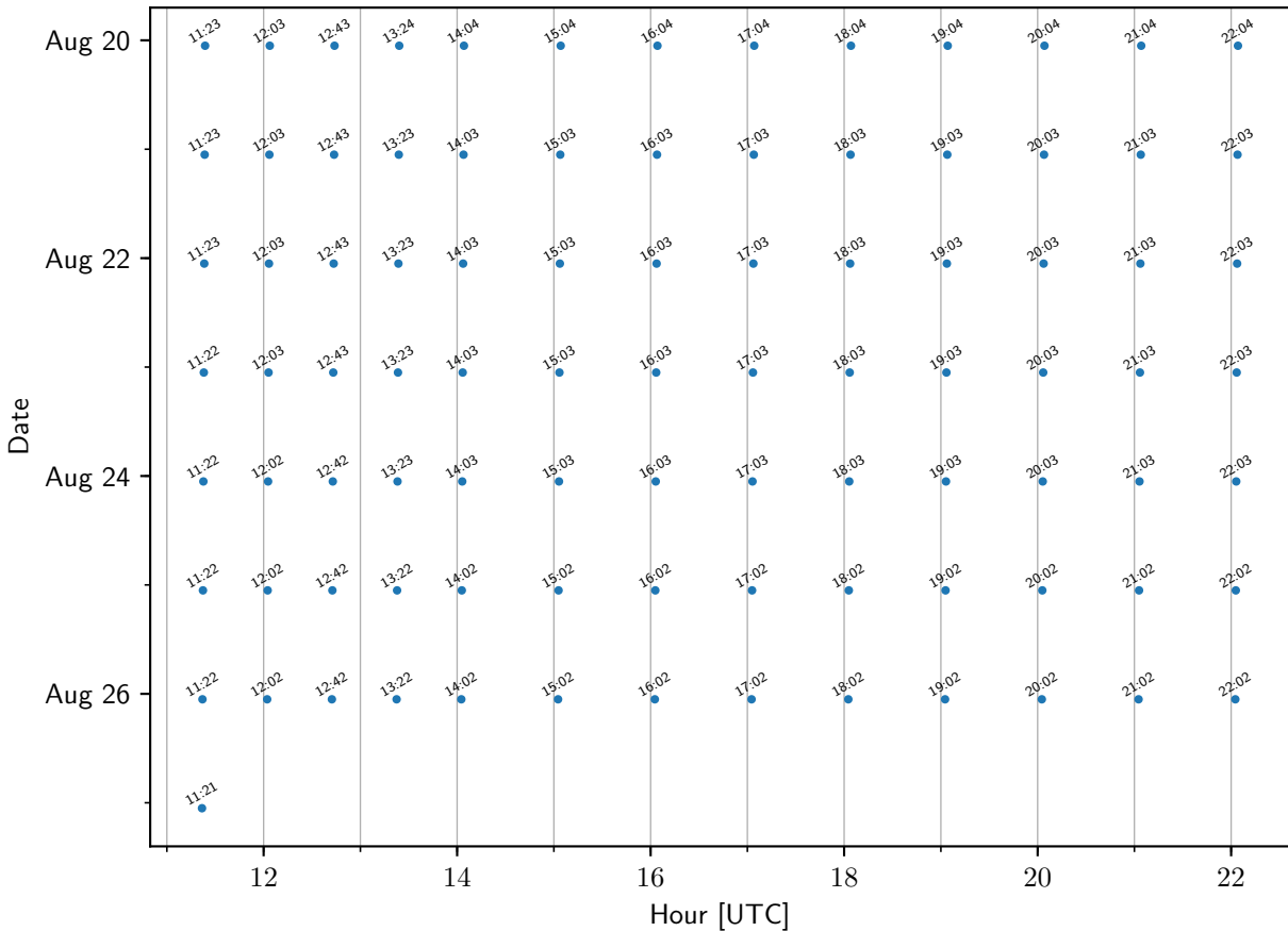
TEMPO sample times: OldFieldNY
