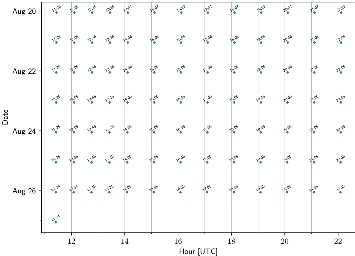
TEMPO sample times: UMCP
