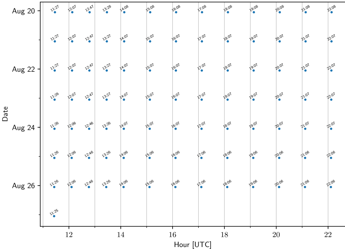
TEMPO sample times: Durham
