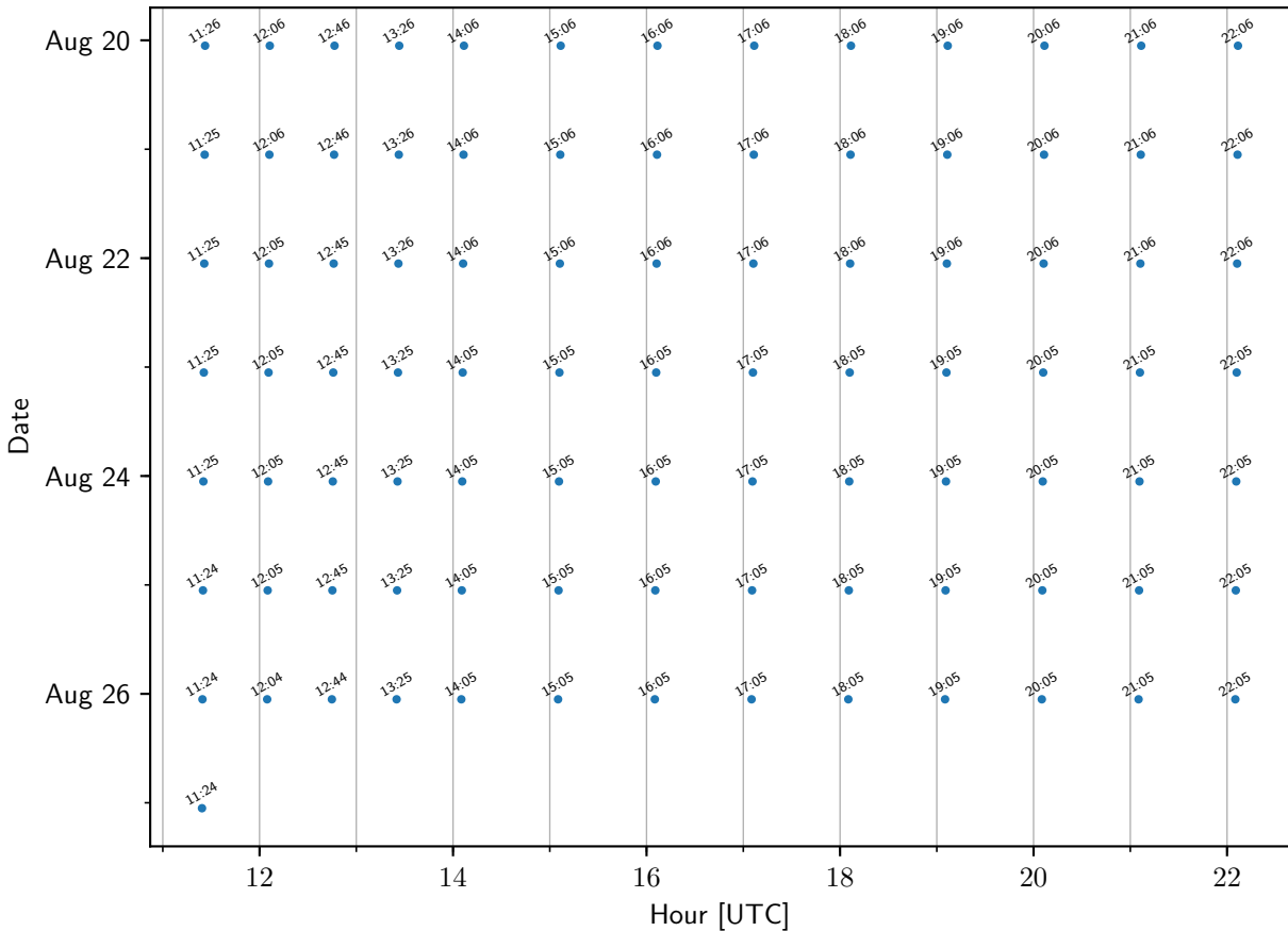
TEMPO sample times: Baltimore
