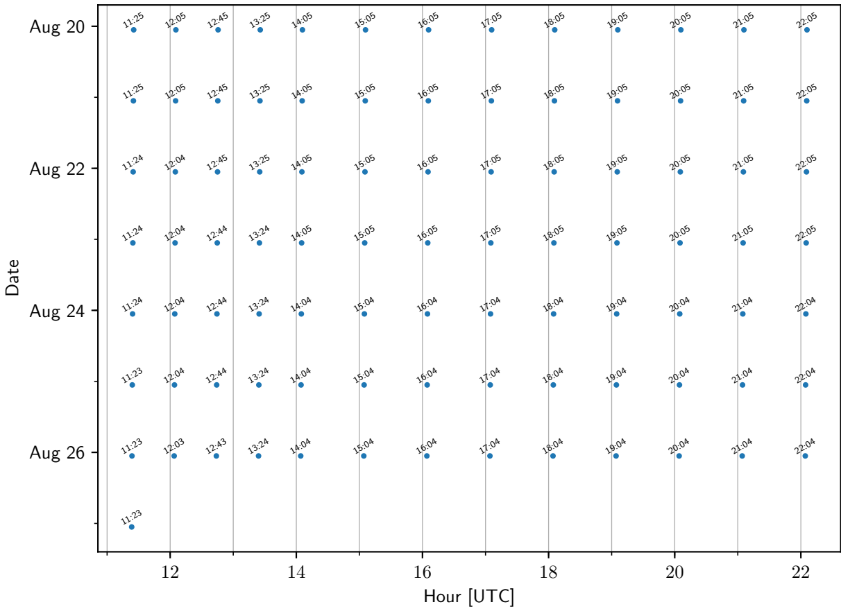
TEMPO sample times: VirginiaBeachVA-CBBT
