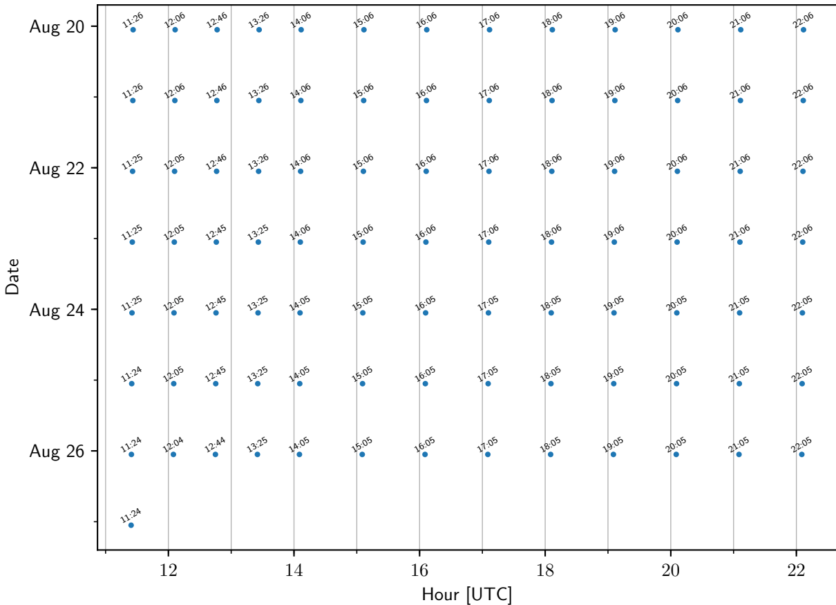
TEMPO sample times: Padonia
