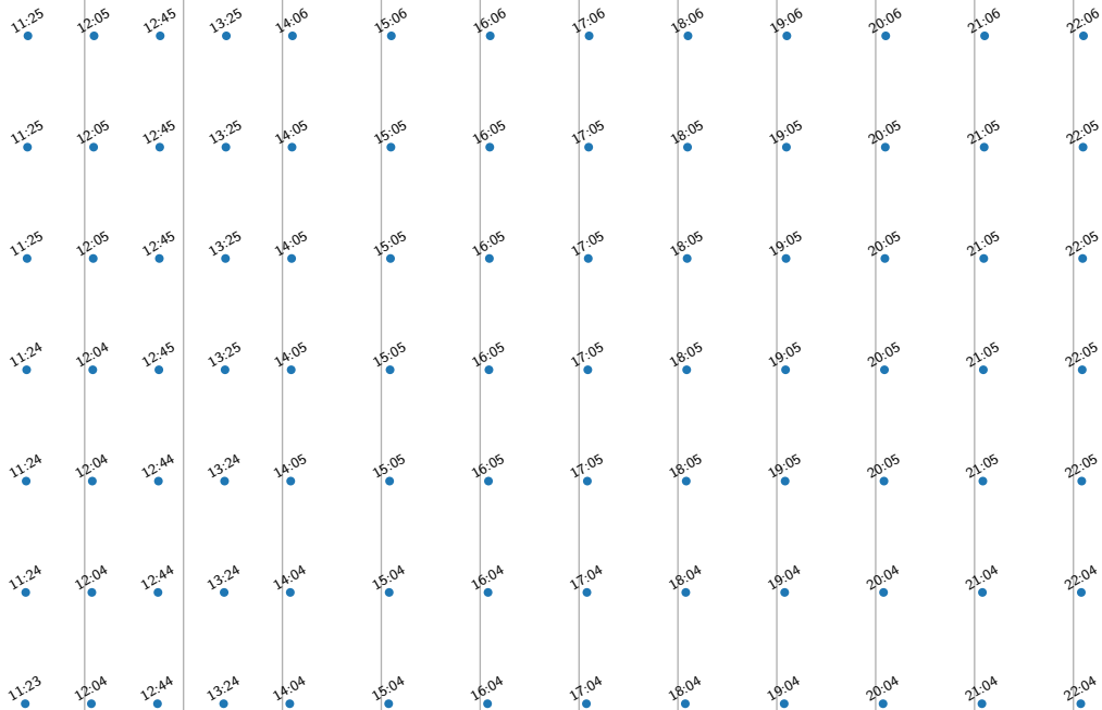
TEMPO sample times: NASA_LaRC
