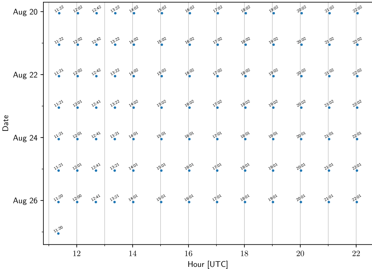
TEMPO sample times: BostonMA
