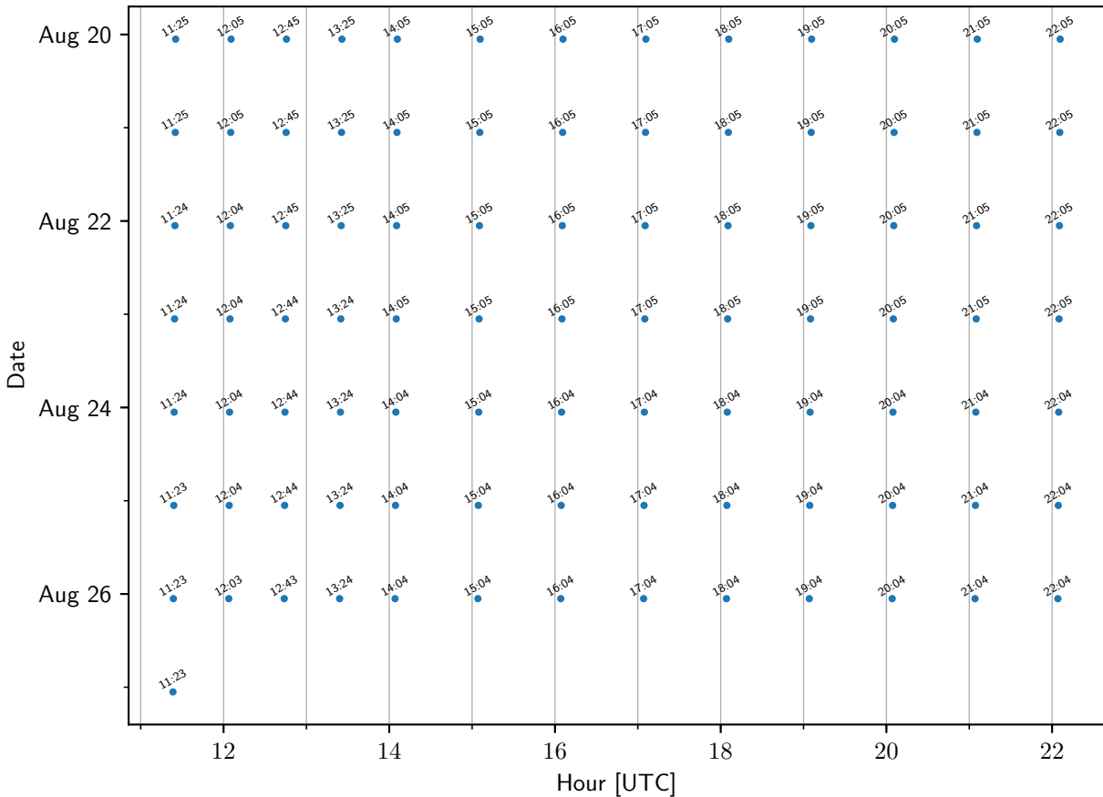
TEMPO sample times: CBBT
