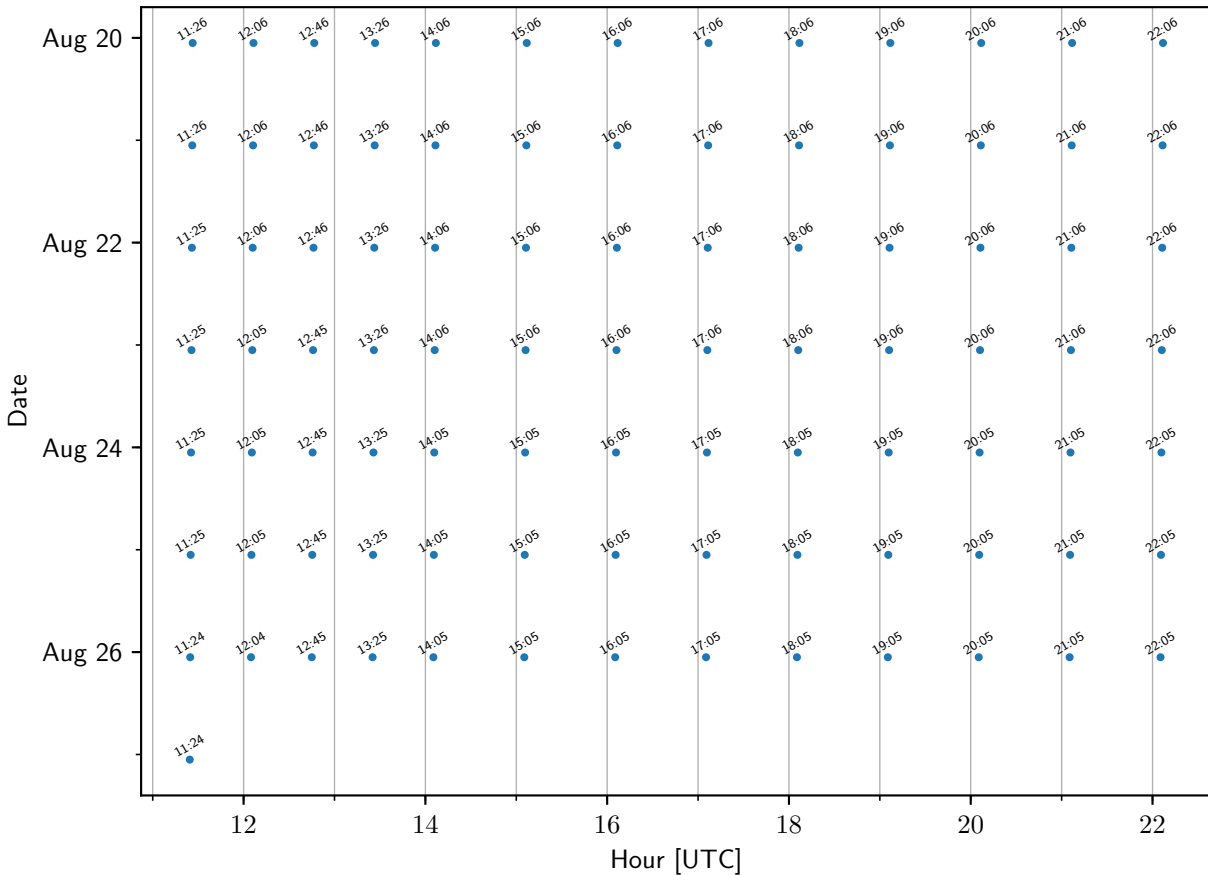
TEMPO sample times: NASA_GSFC
