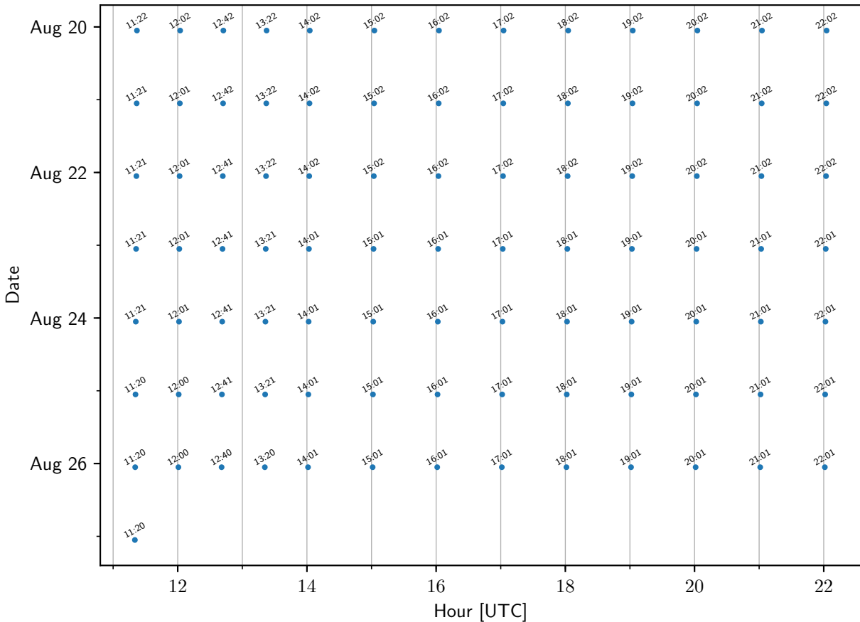
TEMPO sample times: CapeElizabethME
