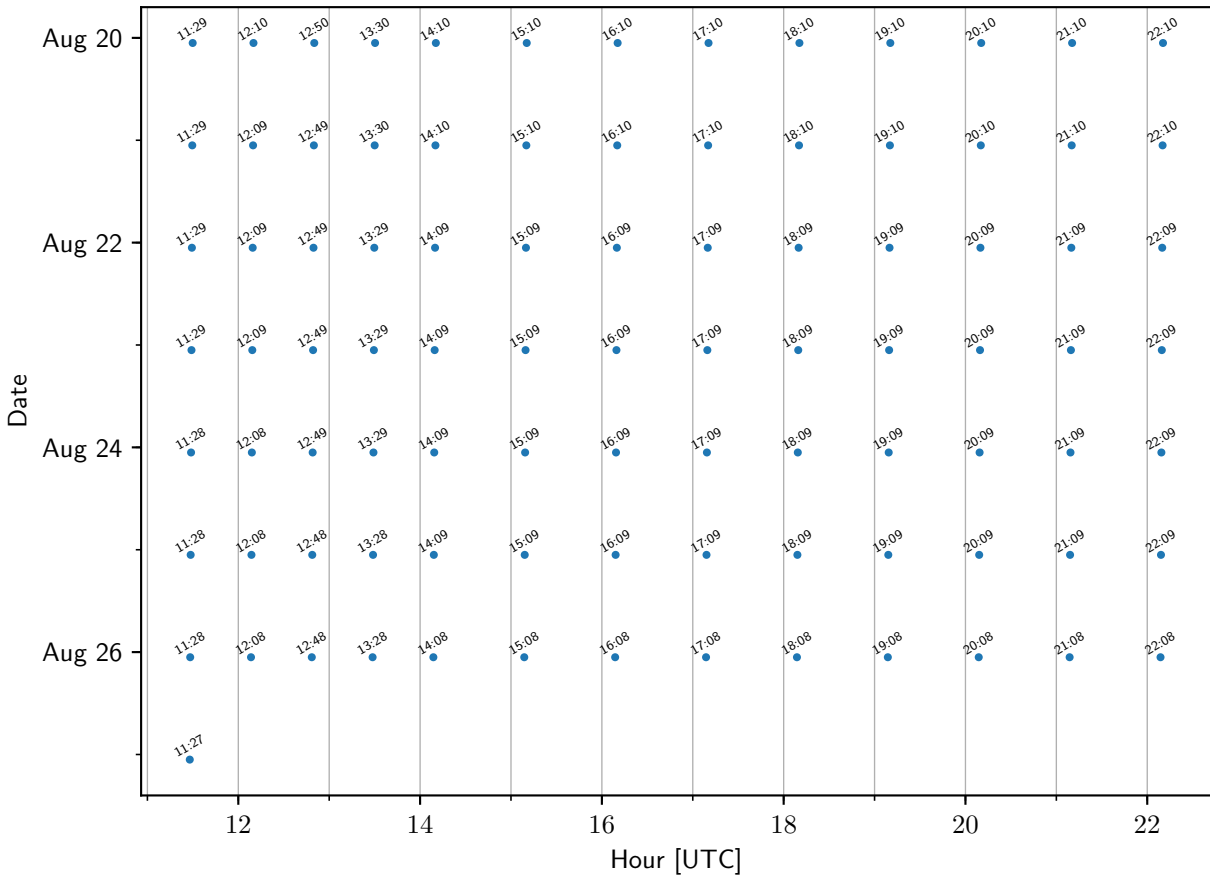
TEMPO sample times: Egbert
