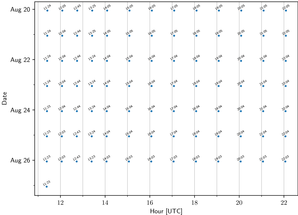
TEMPO sample times: WallopsIslandVA
