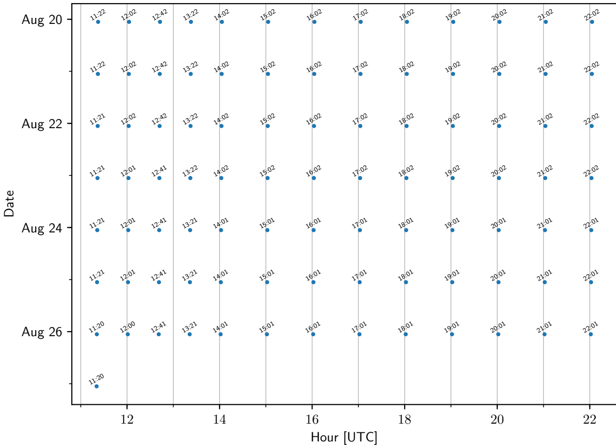
TEMPO sample times: Harvard
