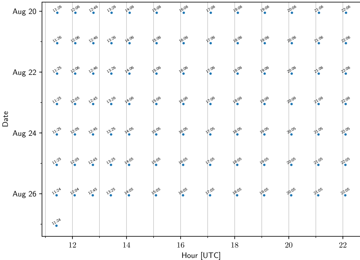
TEMPO sample times: CollegePark
