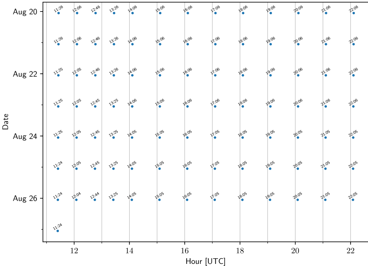
TEMPO sample times: SevernMD
