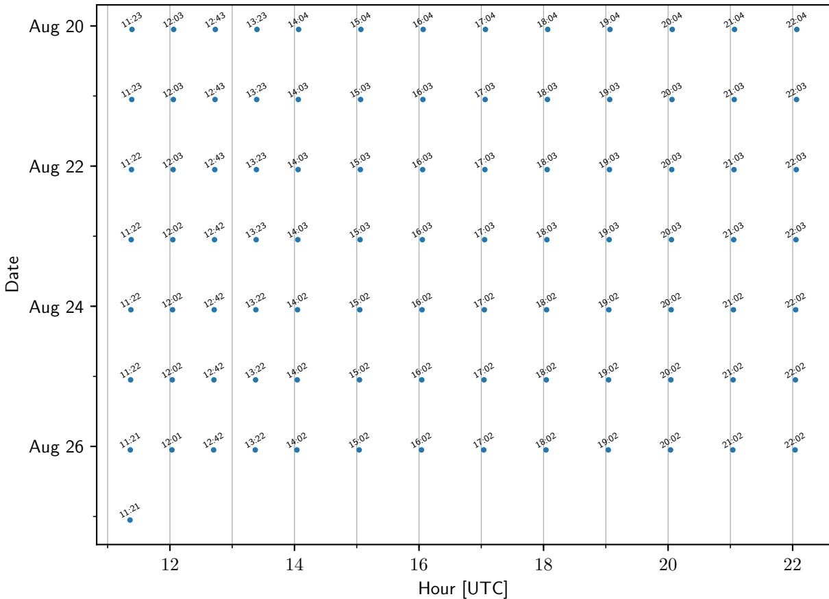
TEMPO sample times: BranfordCT
