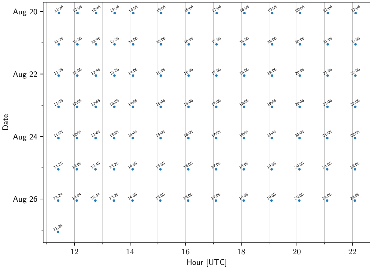
TEMPO sample times: ElkridgeMD
