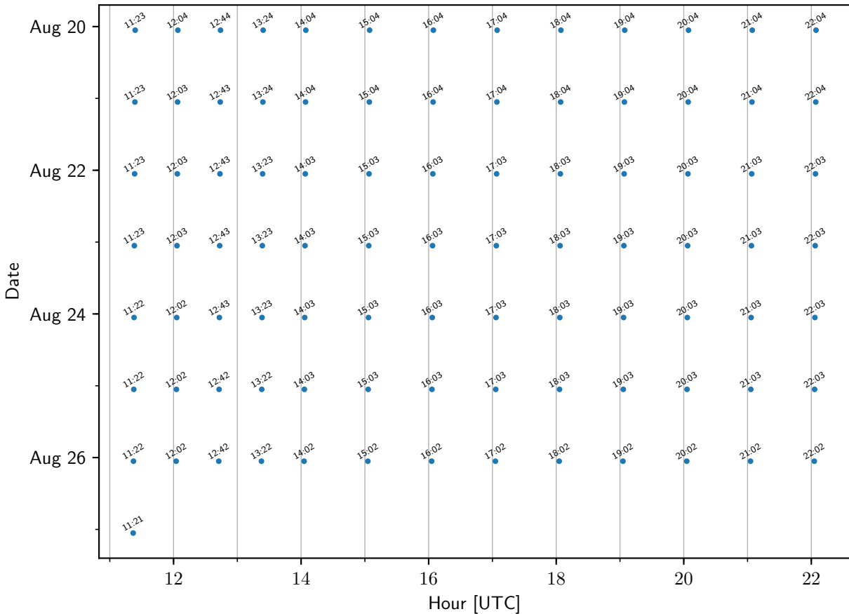
TEMPO sample times: WestportCT
