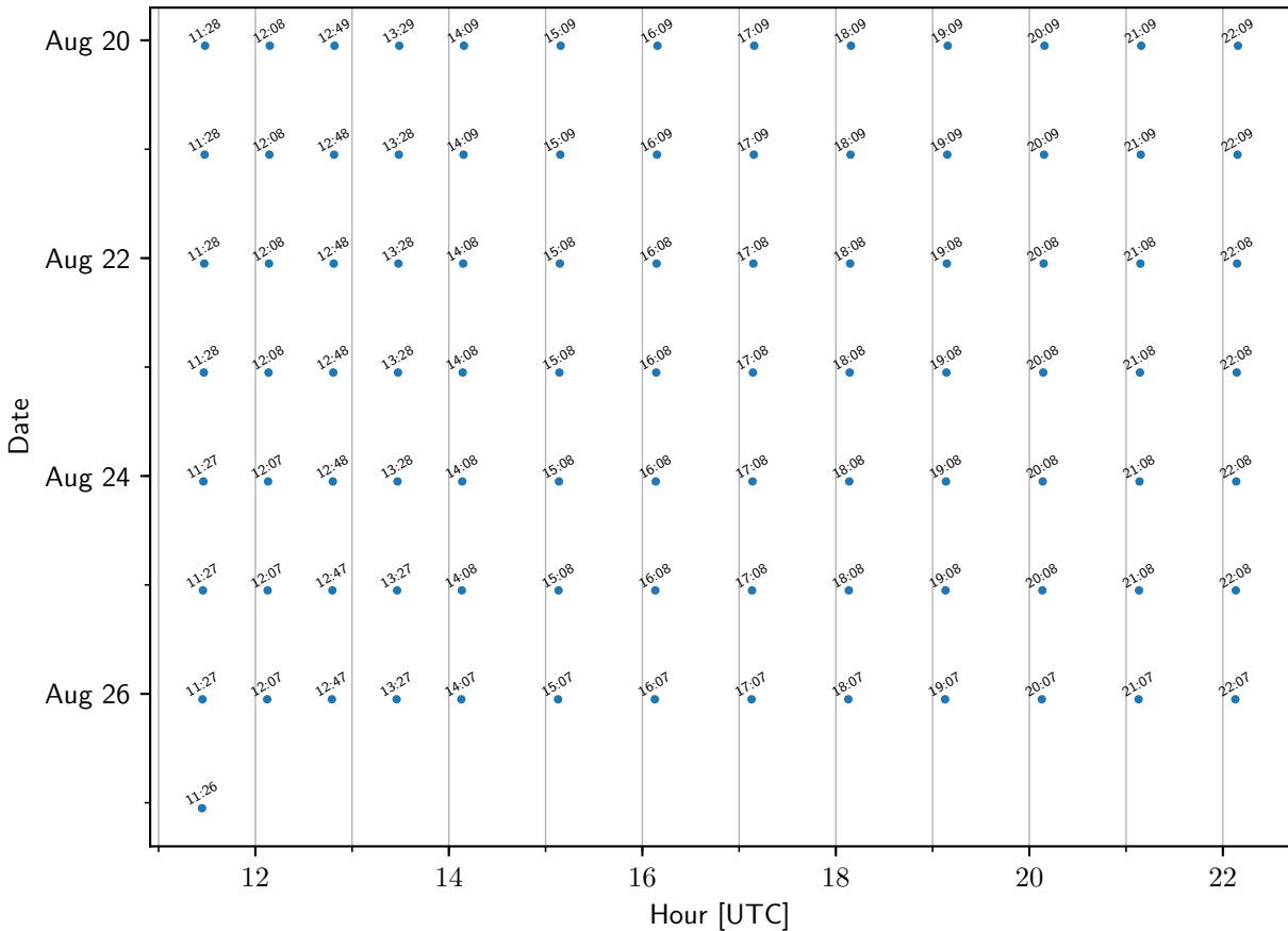
TEMPO sample times: BuffaloNY
