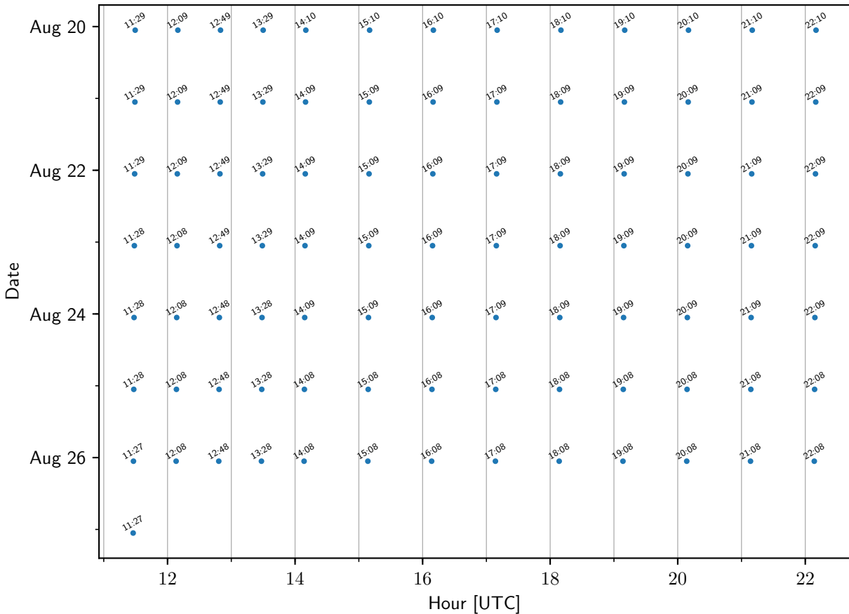
TEMPO sample times: Toronto-West
