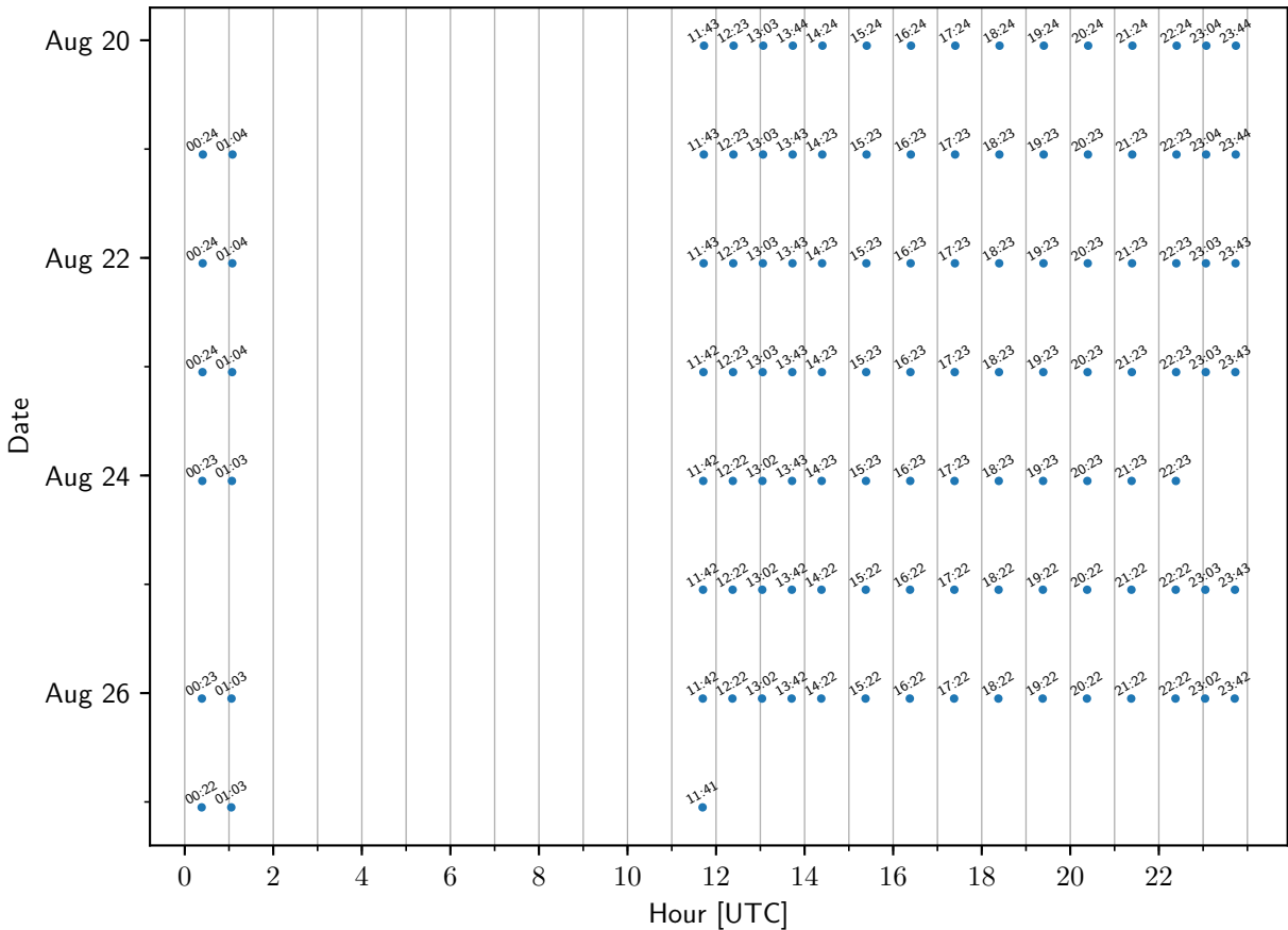
TEMPO sample times: HoustonTXMoodyTowers
