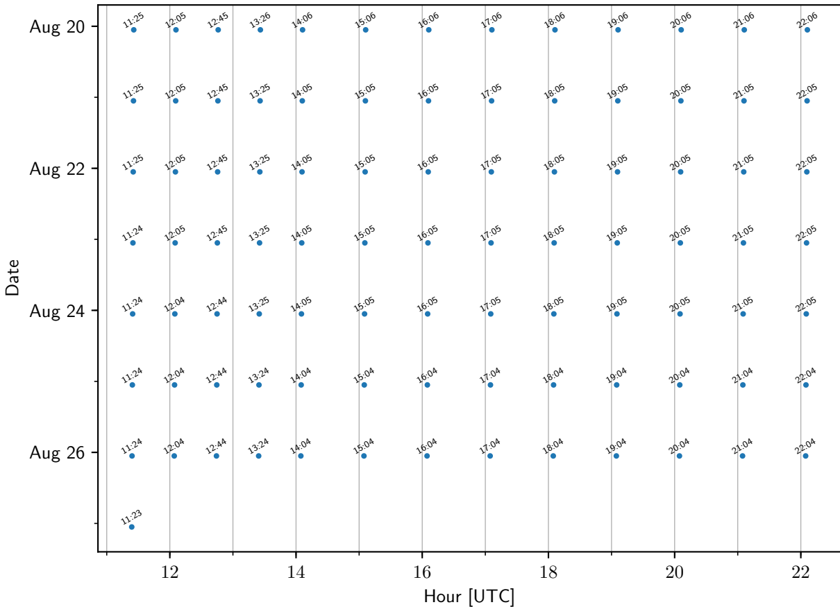
TEMPO sample times: Fairhill
