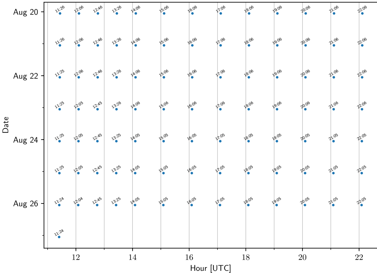
TEMPO sample times: GreenbeltMD
