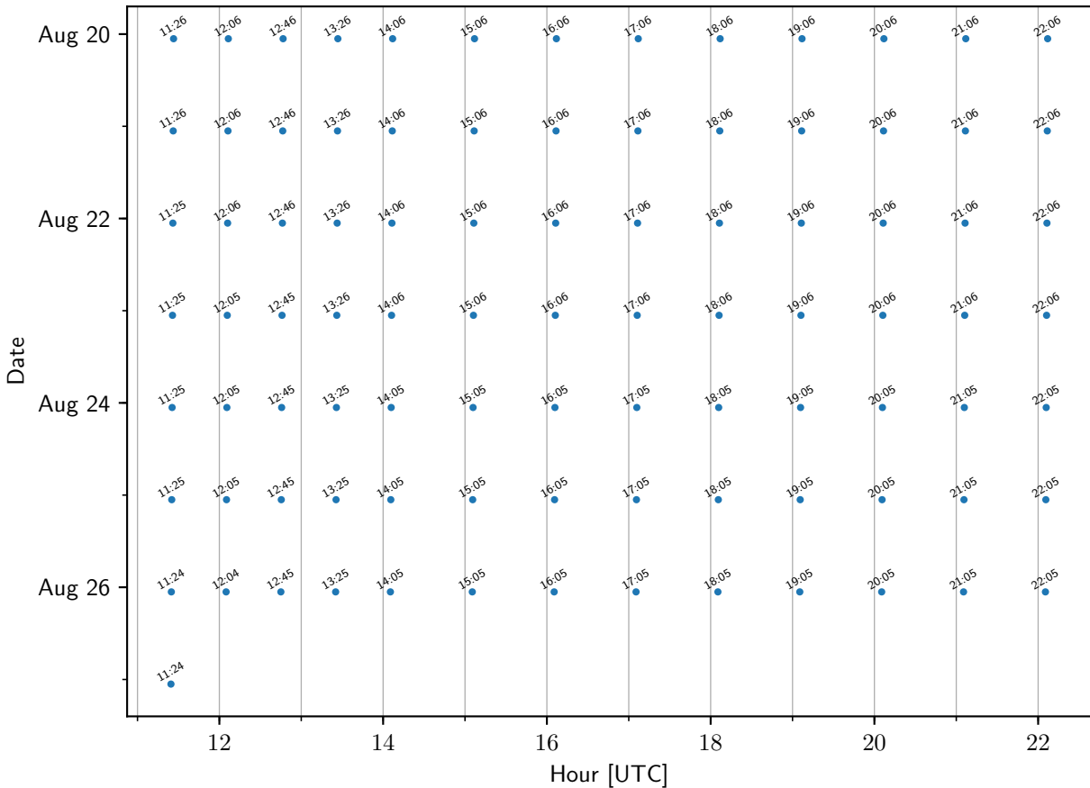
TEMPO sample times: ColumbiaMD
