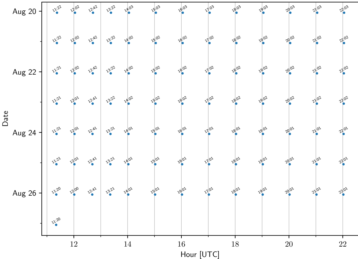
TEMPO sample times: CambridgeMA2
