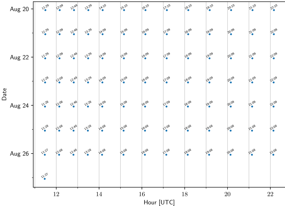
TEMPO sample times: Toronto
