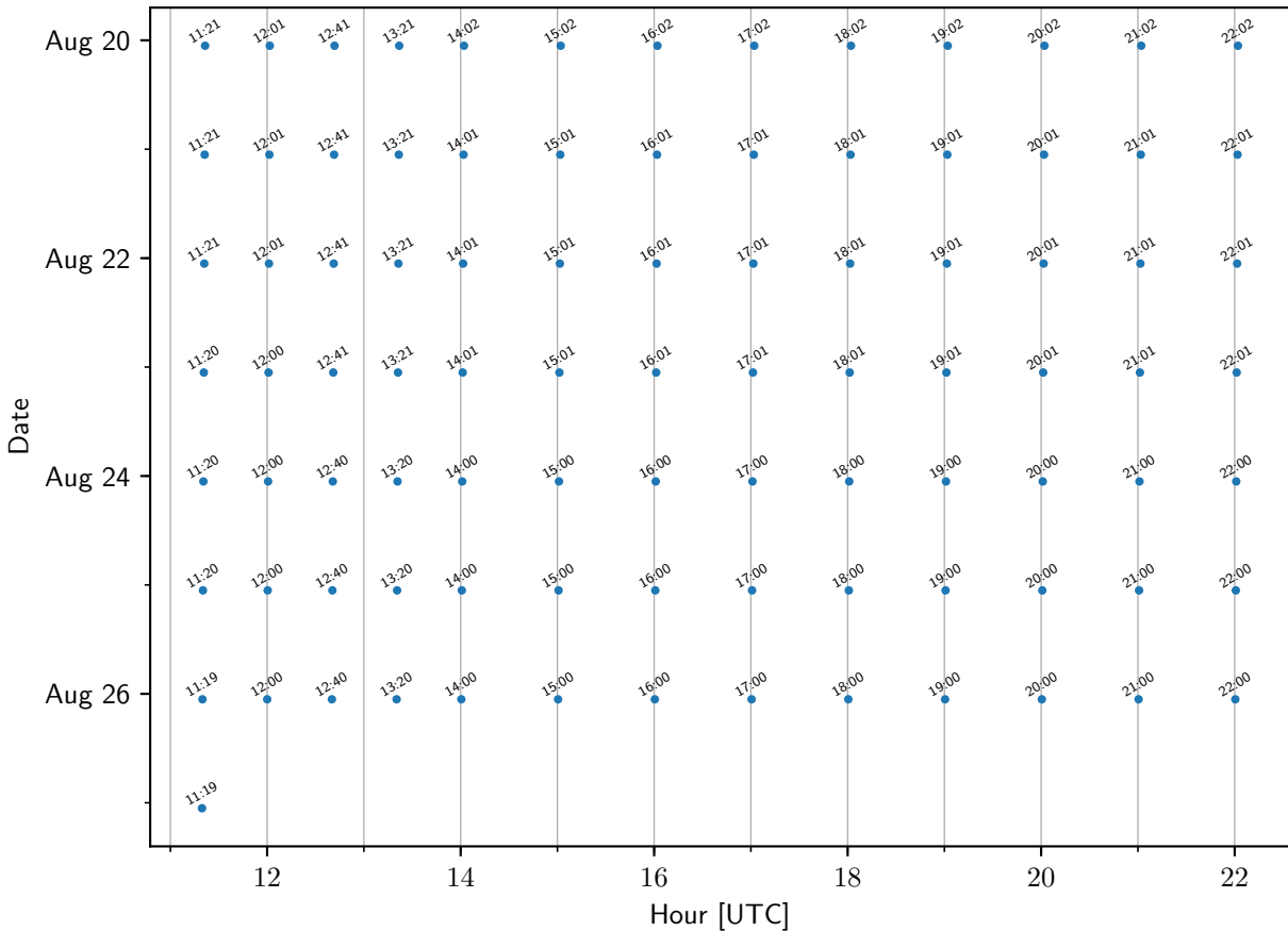
TEMPO sample times: CBM
