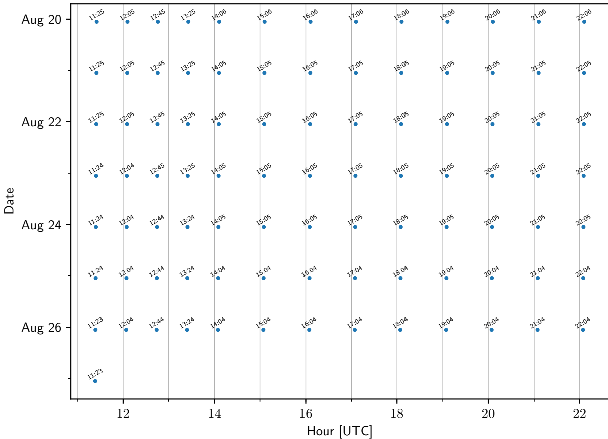
TEMPO sample times: HamptonVA-HU
