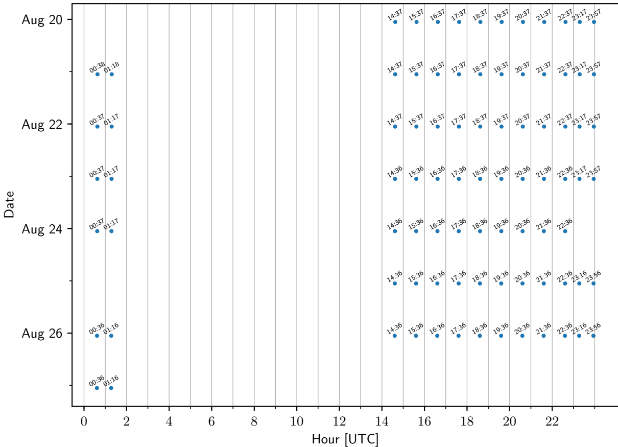
TEMPO sample times: SaltLakeCityUT-Hawthorne
