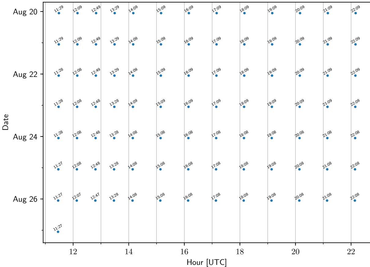
TEMPO sample times: BlacksburgVA
