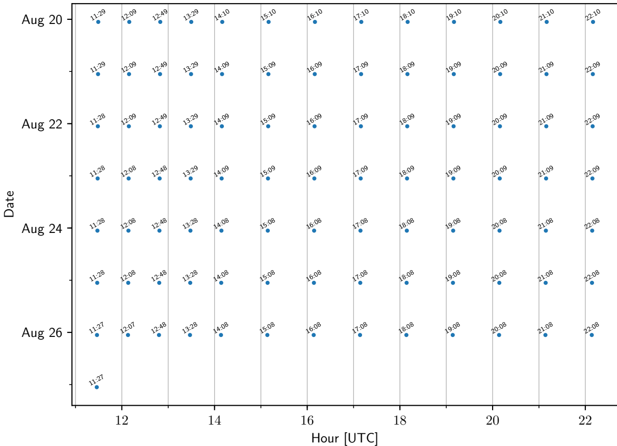
TEMPO sample times: StGeorge
