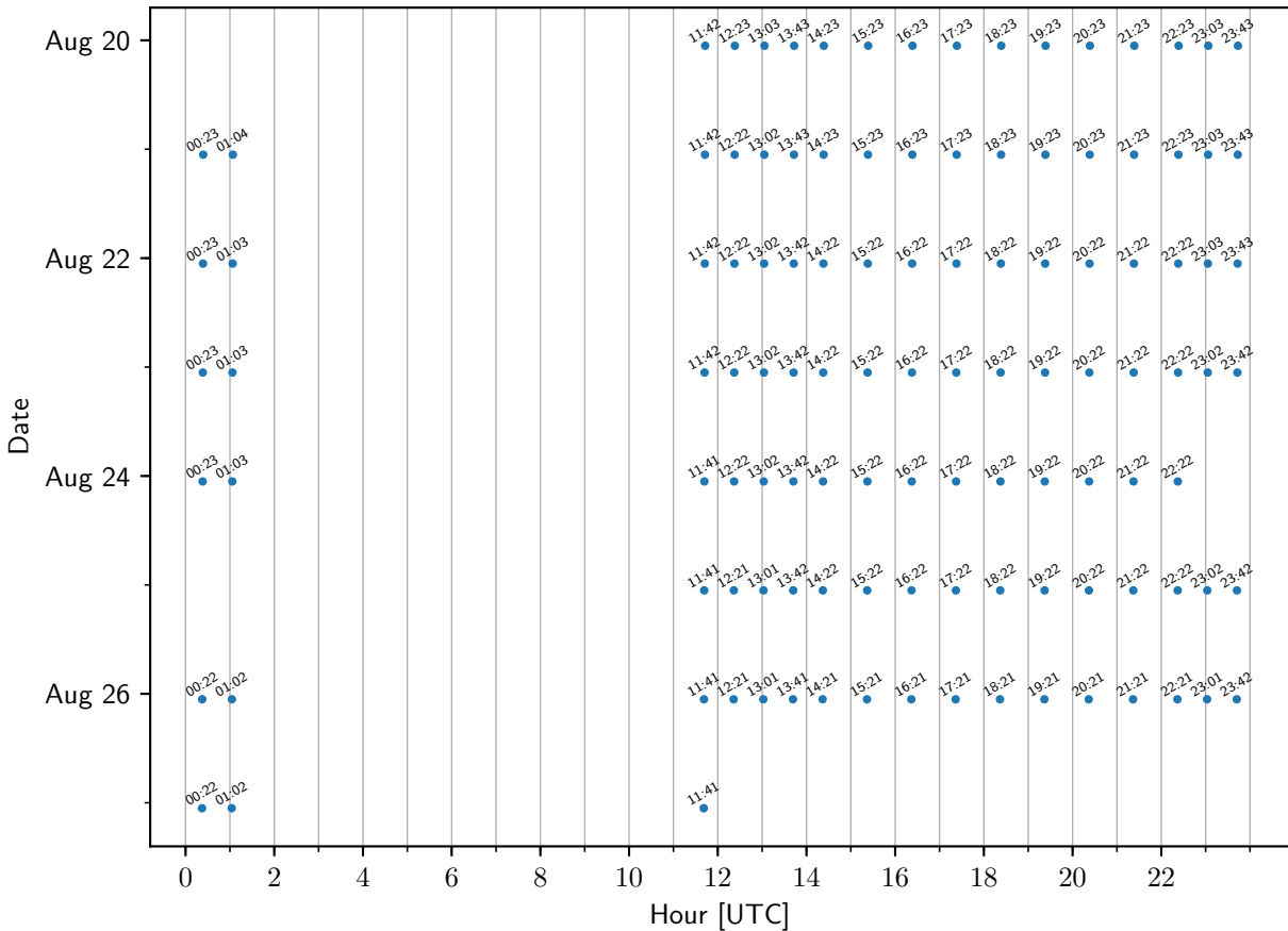
TEMPO sample times: staqs-HoustonGulf
