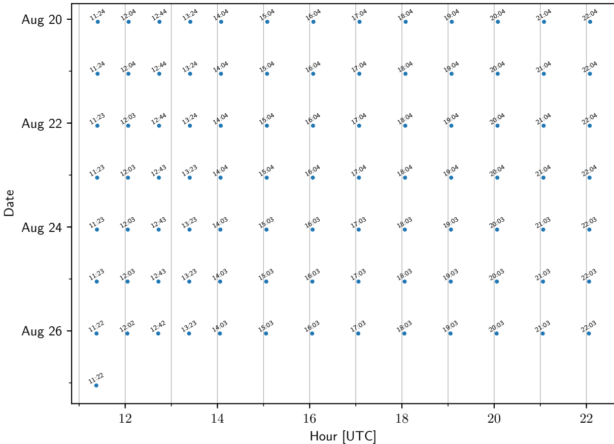
TEMPO sample times: CCNY
