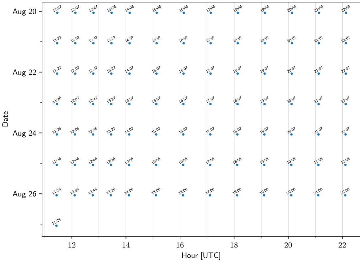
TEMPO sample times: MiamiFL-FIU
