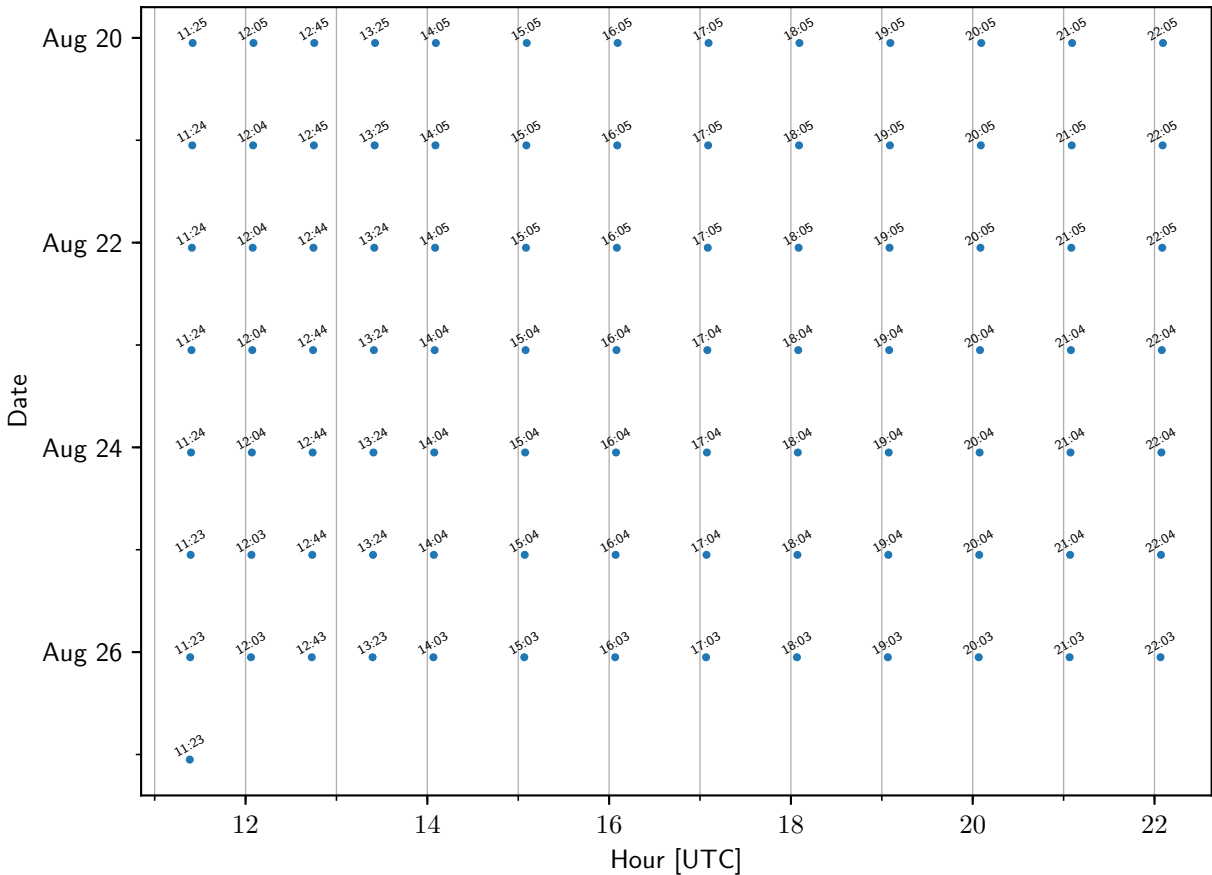
TEMPO sample times: PhiladelphiaPA
