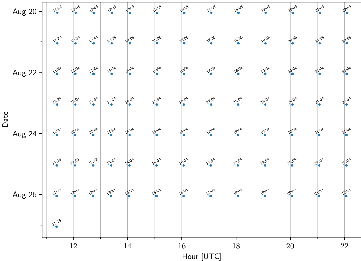
TEMPO sample times: WFF
