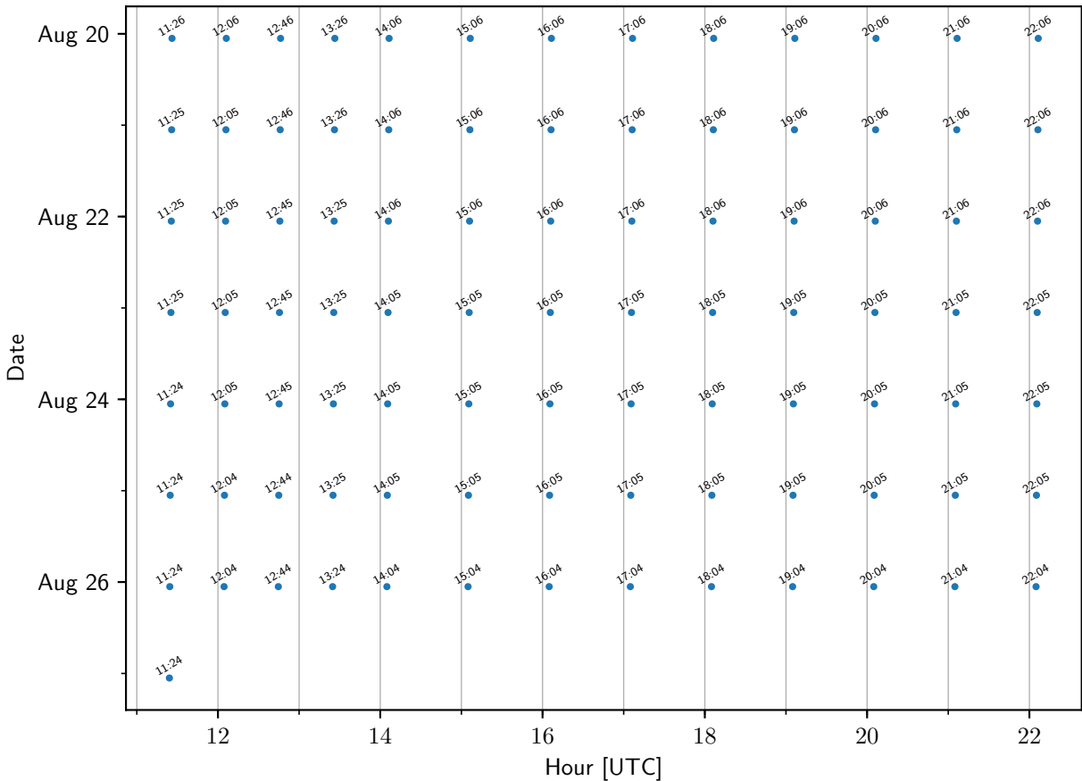
TEMPO sample times: HartMillerIslandMD
