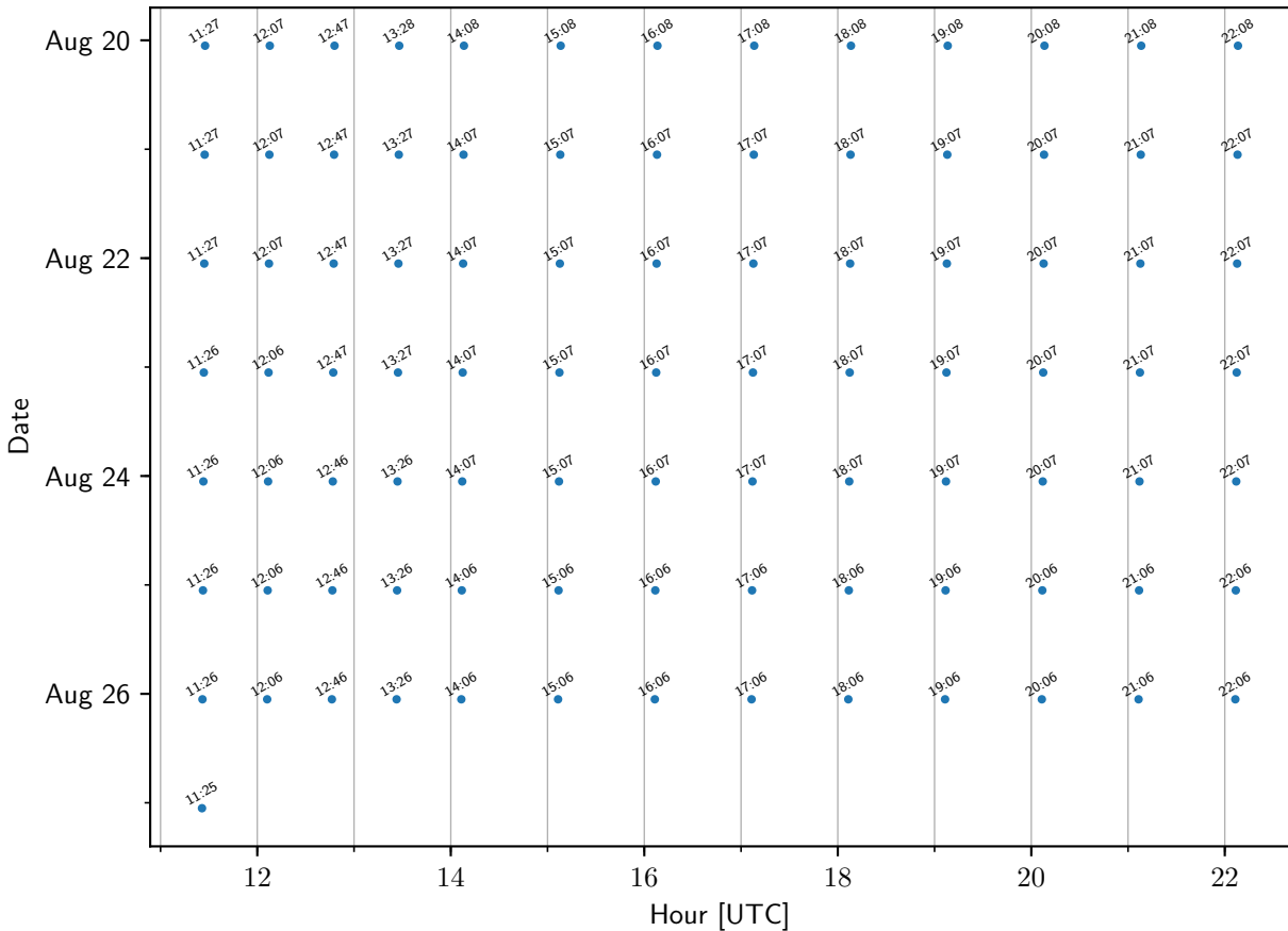
TEMPO sample times: PSU
